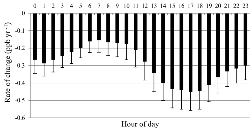
(c) TO in smog season
