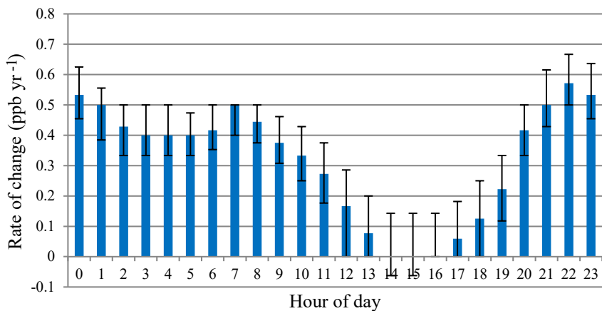
(a) O 3 in smog season
