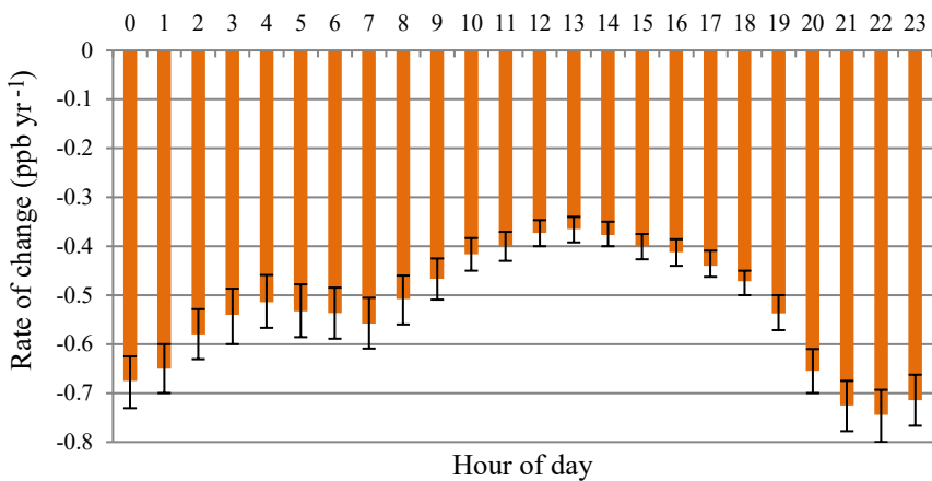
(b) DO 3 in smog season
