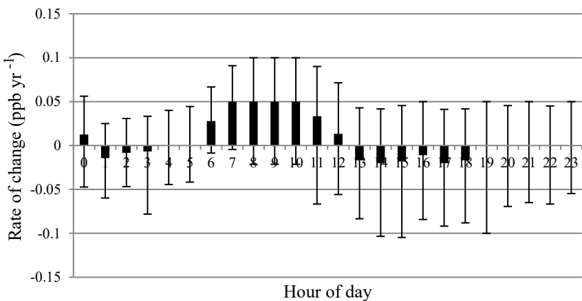
(c) TO
