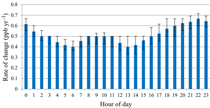
(a) O 3
