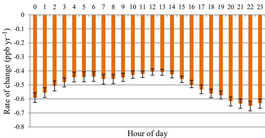
(b) DO 3
