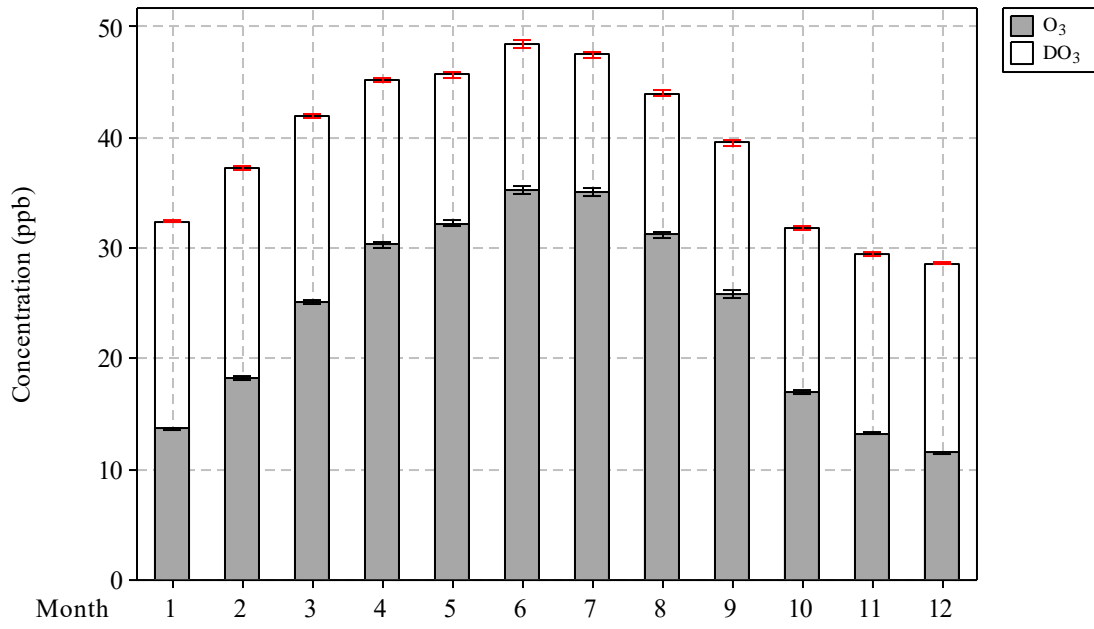
Seasonal variability of O 3 and DO 3 at Windsor during 1996–2015 95 % CI for the mean
