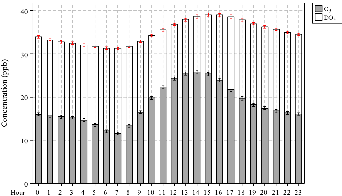
(c) Non-smog season diurnal variability of O 3 and DO 3 at Windsor during 1996–2015
