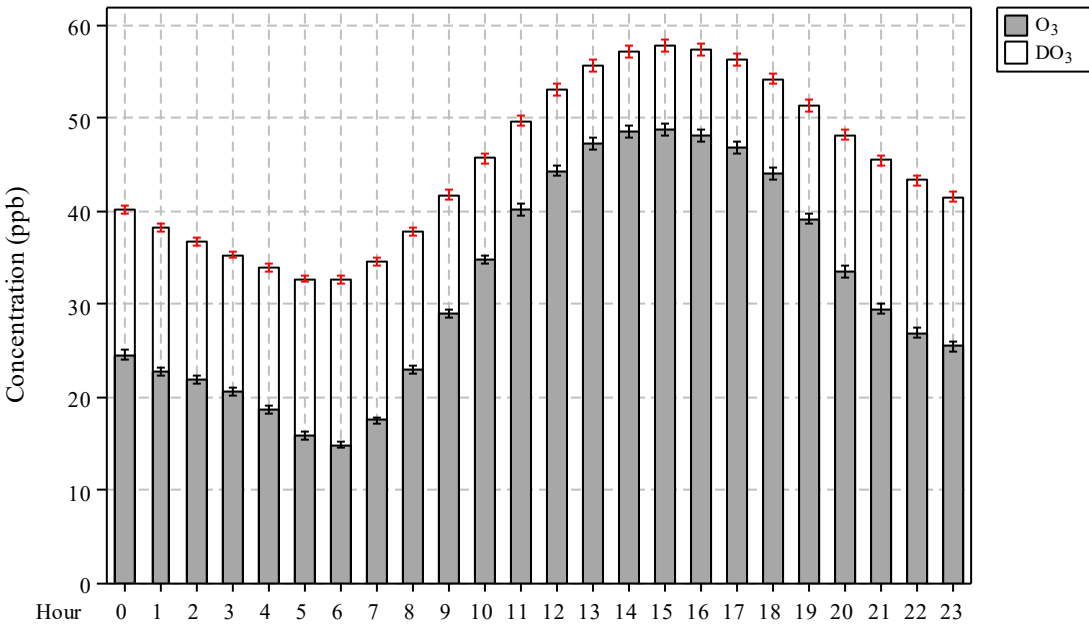
(b) Smog season diurnal variability of O 3 and DO 3 at Windsor during 1996–2015
