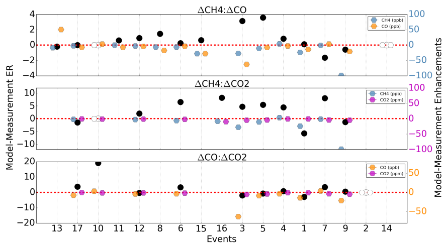
Figure S9. Difference between modelled and measured enhancement ratio (ER, black dots) and enhancement (coloured markers) for the species that showed coincident enhancements. Positive values indicate model overestimates and the negative values represent model underestimates. The white markers represent enhancements and ERs where the model failed to capture the measured values. Units for the ERs are same as in Table S6.
