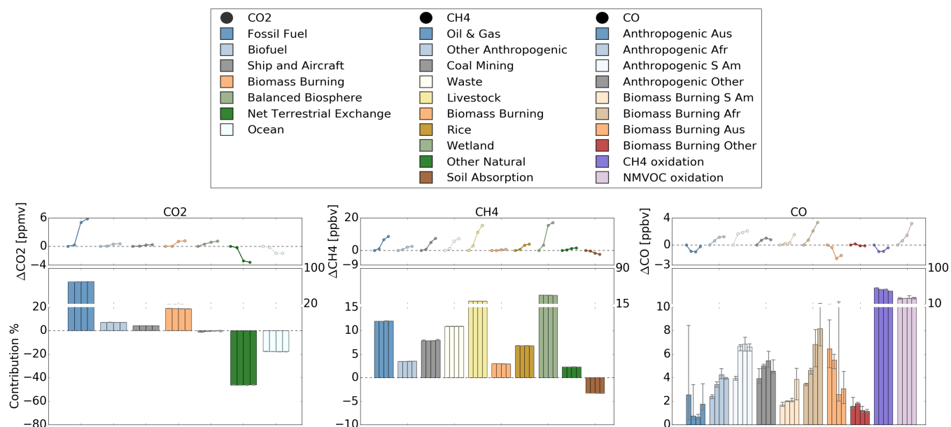
Figure S6. CO 2 , CH 4 and CO tracer contribution across the 4 measurement section in 2012 and 2013 (2012 NB, 2012 2B, 2013 NB, 2013 SB, from left to right) for the total amount of each gas.
