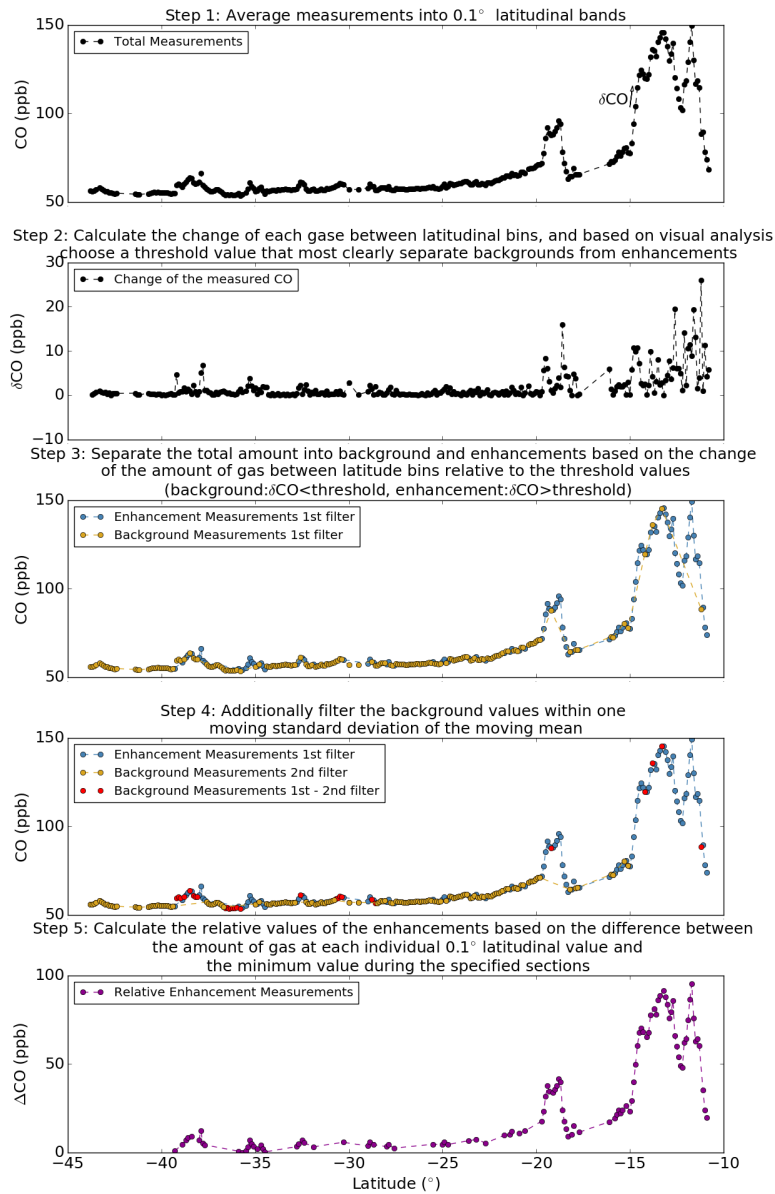
Figure S5. The separation process of the measured and modelled data into background values and enhancements. We use CO from the 2013 NB section as an example. The threshold values for each gas used during the separation can be found in Table S3.
