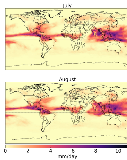
Figure S3. Position of the ITCZ and SPCZ during July and August 2013 based on total convective precipitation at the ground from MERRA2 meteorology processed with the GEOS-Chem model.
