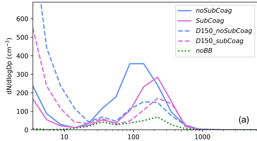
JJA average size distributions (modeled Alaska)
