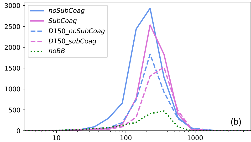
ASO average size distributions (modeled Amazon)
