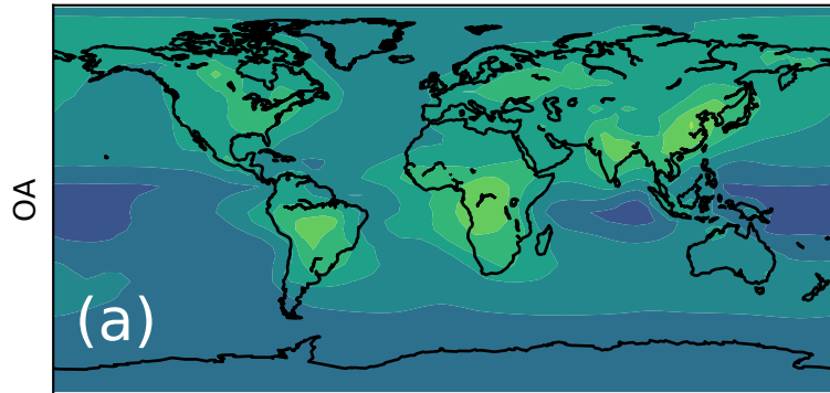
Total column mass
