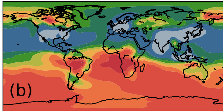
Percent due to biomass burning
