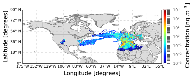
(b) Leipzig, 31 March, 23:00, layer corresponding to L2
