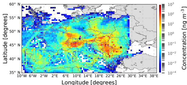
(c) Pillersdorf, 02 April, 06:00, layer L2, zoomed
