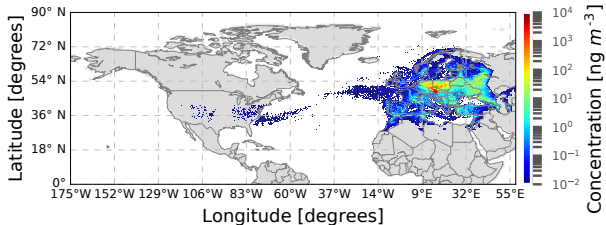
(a) Pillersdorf, 02 April, 06:00, layer L1
