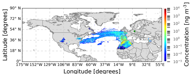
(b) Leipzig, 31 March, 18:00, layer corresponding to L1
