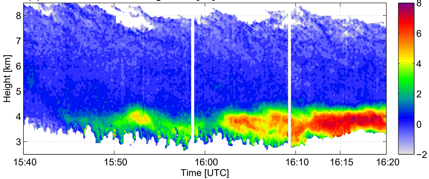
(b) 35 / 94 GHz dual-wavelength ratio [dB]
