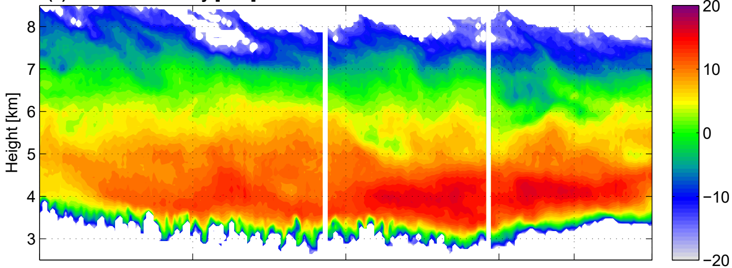
(a) 35 GHz reflectivity [dBZ]
