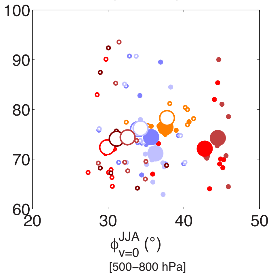
(b) JJA \phi_{v=0} - \chi_{\text{CO}} ( r = -0.0013 )
