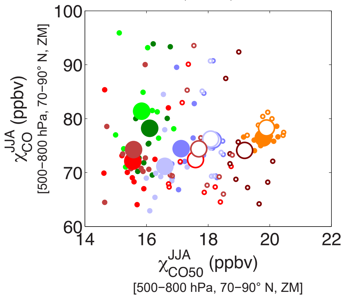
(a) JJA \chi_{\text{CO50}} - \chi_{\text{CO}} ( r = 0.12 )
