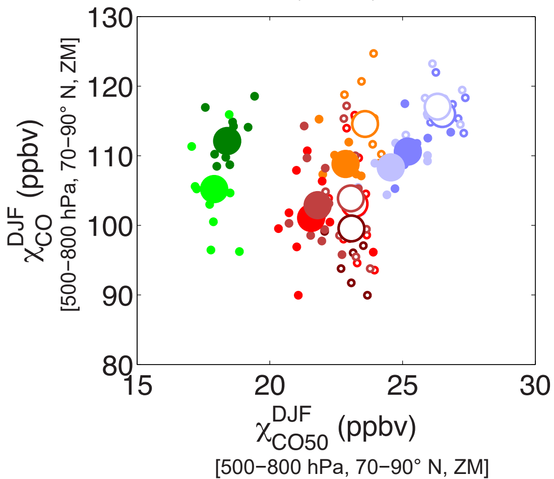
(c) DJF \chi_{\text{CO50}} - \chi_{\text{CO}} ( r = 0.42 )
