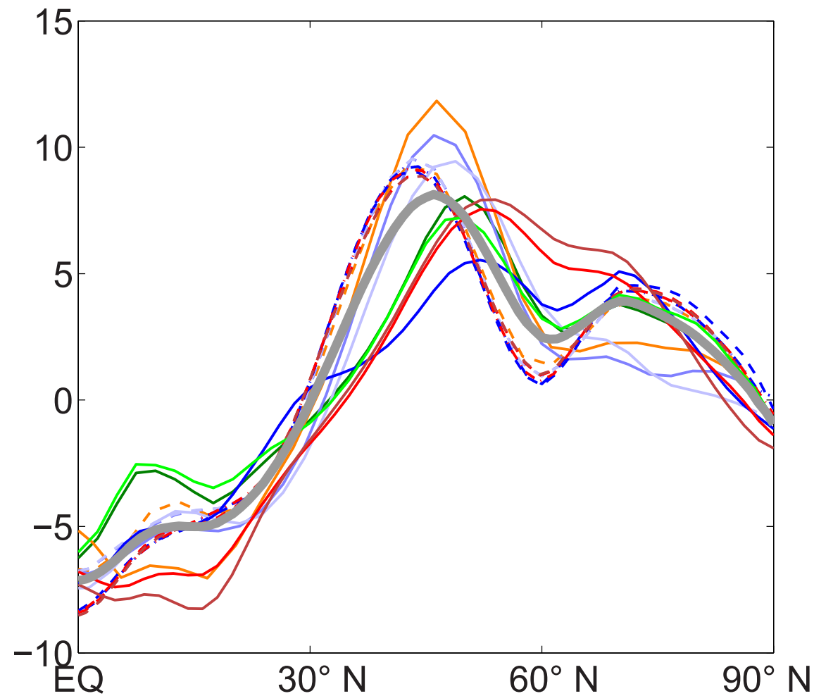
(b) JJA
