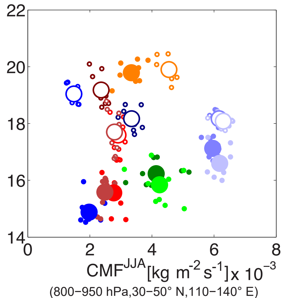
(b) JJA CMF- \chi_{\text{CO50}}
