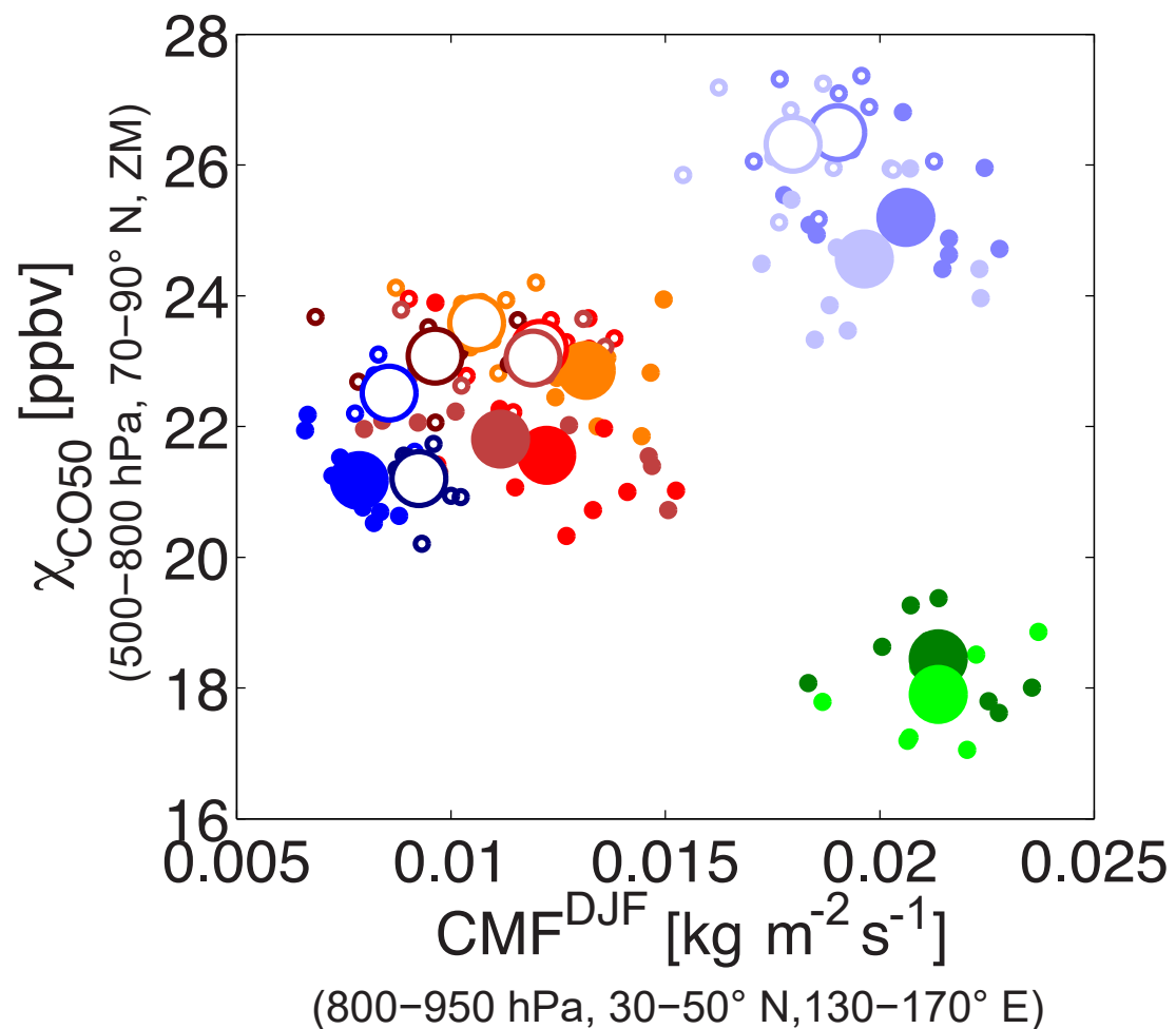
(a) DJF CMF- \chi_{\text{CO50}}
