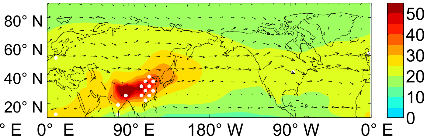
(f) JJA
