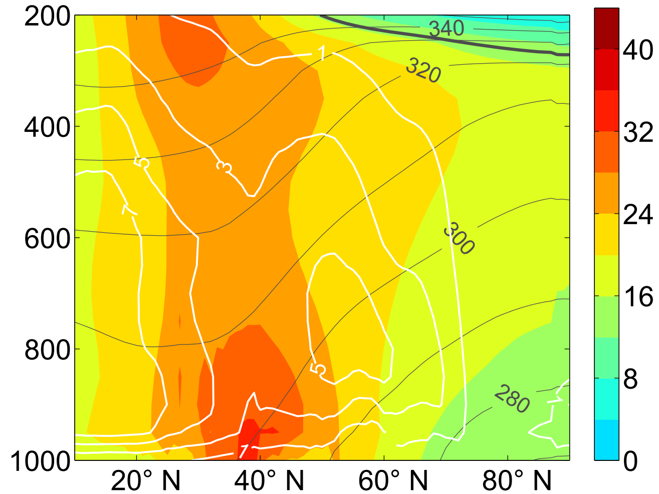
(f) JJA
