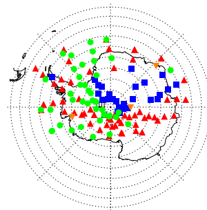
(c) MIPAS: 2011-06-25
