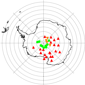
CLaMS: 2011-06-25
