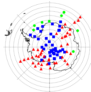
CLaMS: 2011-07-06
