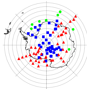
(f) CLaMS: 2011-07-06
