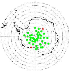
(a) MIPAS: 2011-05-25
