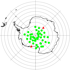
MIPAS: 2011-06-25
