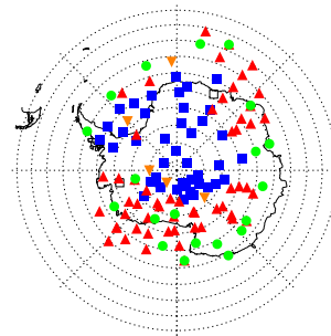
(e) MIPAS: 2011-07-06
