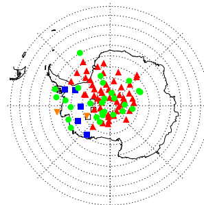
MIPAS: 2011-09-08
