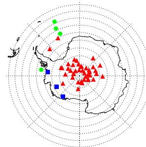
CLaMS: 2011-09-08
