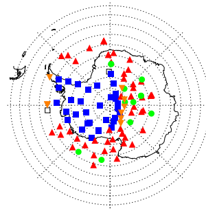
(g) MIPAS: 2011-08-21
