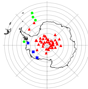
(j) CLaMS: 2011-09-08
