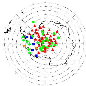
(i) MIPAS: 2011-09-08
