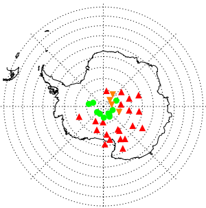
(b) CLaMS: 2011-05-25
