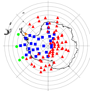
(h) CLaMS: 2011-08-21
