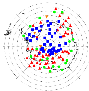
MIPAS: 2011-07-06
