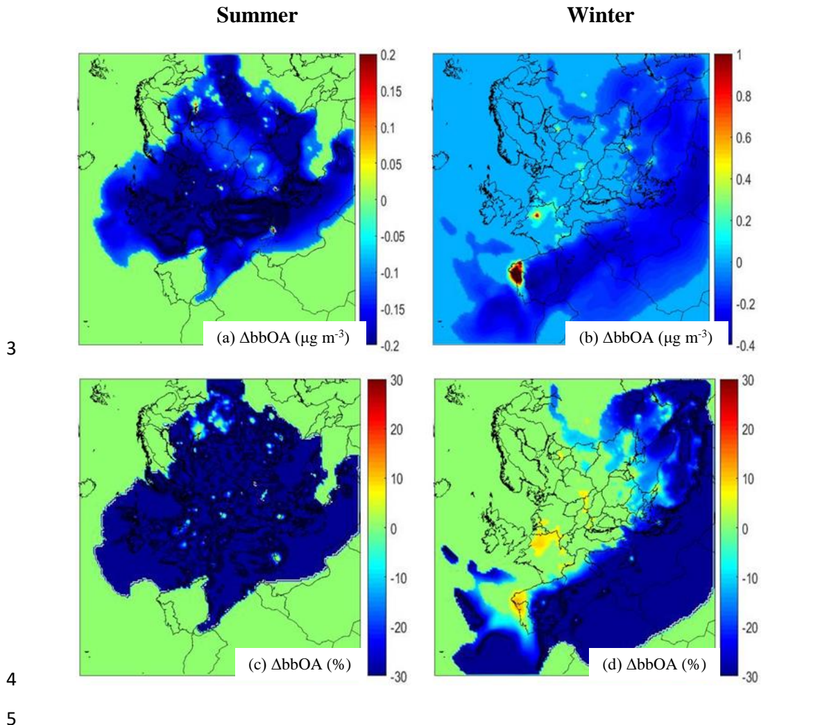
6 Figure S4. Average predicted absolute ( \mu\text{g m}^{-3} ) change of ground-level \text{PM}_{2.5} total 7 bbOA concentrations from PMCAMx-SR base case and sensitivity simulations during 8 the modeled summer and winter periods (a-b). Also shown the corresponding relative 9 (%) change of ground-level \text{PM}_{2.5} total bbOA concentrations during the modeled 10 periods (c-d). Positive values indicate that PMCAMx-SR sensitivity run predicts 11 higher concentrations.
