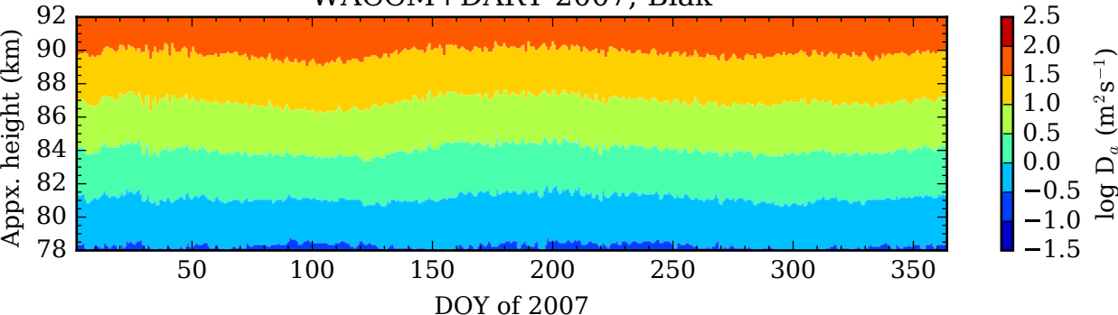
WACCM+DART-2007; Biak
