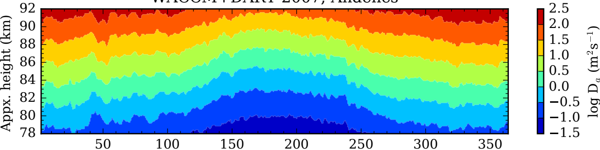
WACCM+DART-2007; Juliusruh
