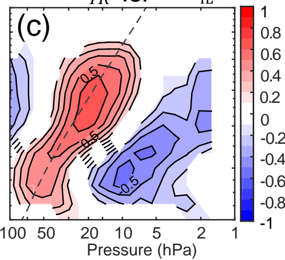
w_{TR} vs. \bar{w}_{TL}^*
