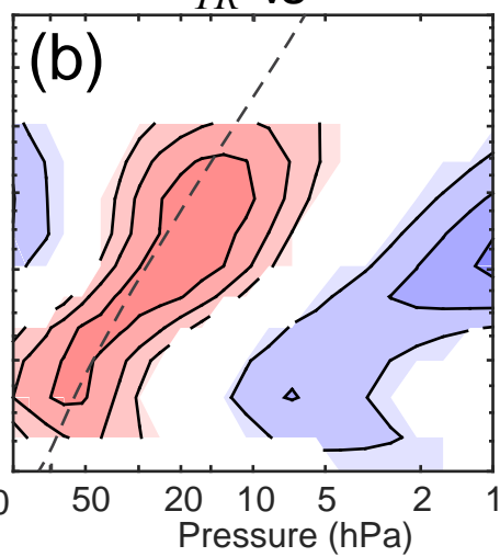
w_{TR} vs. \bar{w}^*
