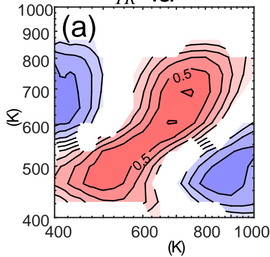
w_{TR} vs. \mathcal{M}
