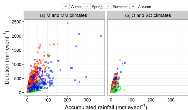
Figure 4. Rainfall duration vs. accumulated rainfall across seasons for each marked rainfall event at Mediterranean (M) and Mediterranean–mountain (MM) stations (a) and at oceanic (O) and semi-oceanic (SO) stations (b).
