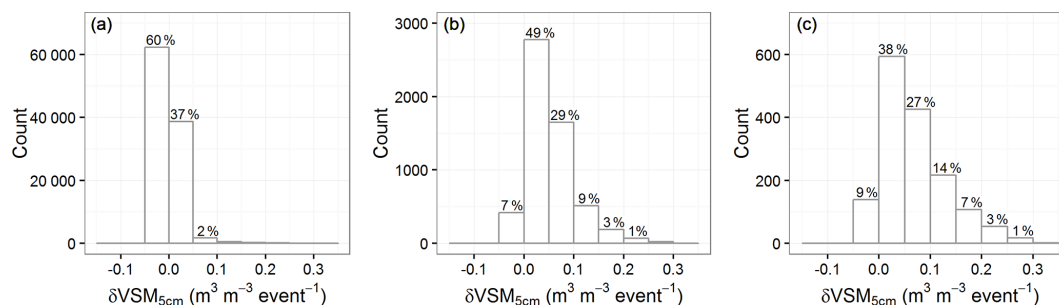
Figure 9. Statistical distribution of \delta VSM_{5cm} for 104 178 fully documented rainfall events (a), 5714 marked rainfall events (b), and 1577 marked rainfall events affecting topsoil temperature (c) defined in Table 2.
