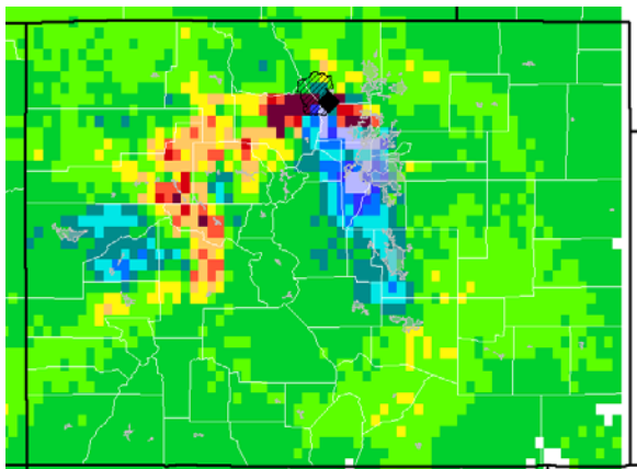
(c) Isoprene
