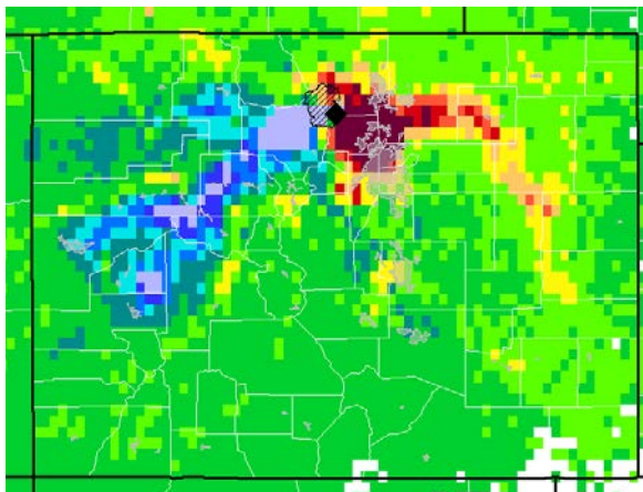
(a) Ethane
