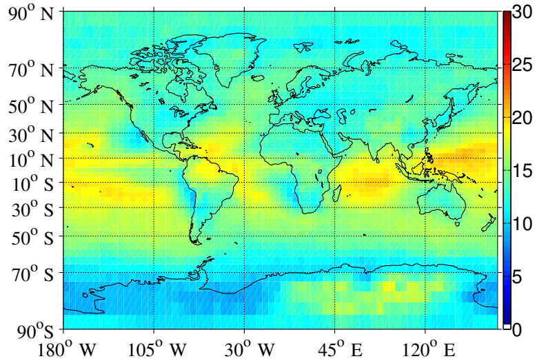
(b) MODIS mean liquid water cloud droplet effective radius ( \mu\text{m} ) daytime, 2008
