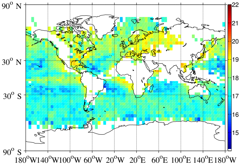
(a) CALIOP median “unobstructed” opaque water cloud lidar ratio S_c (sr) nighttime, 2008
