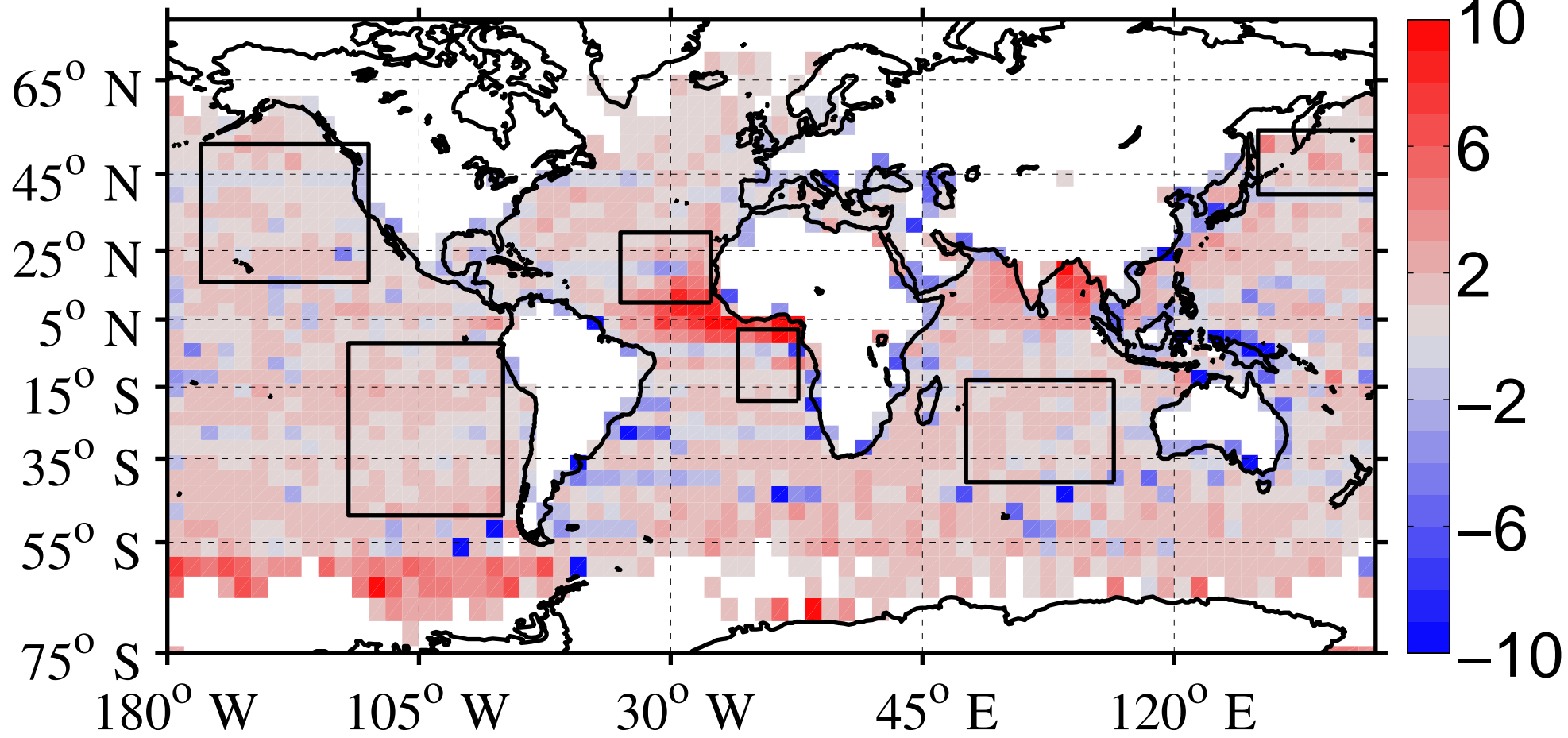
DJF min: -27 max: 5 median: 0.97 mean: 0.64
