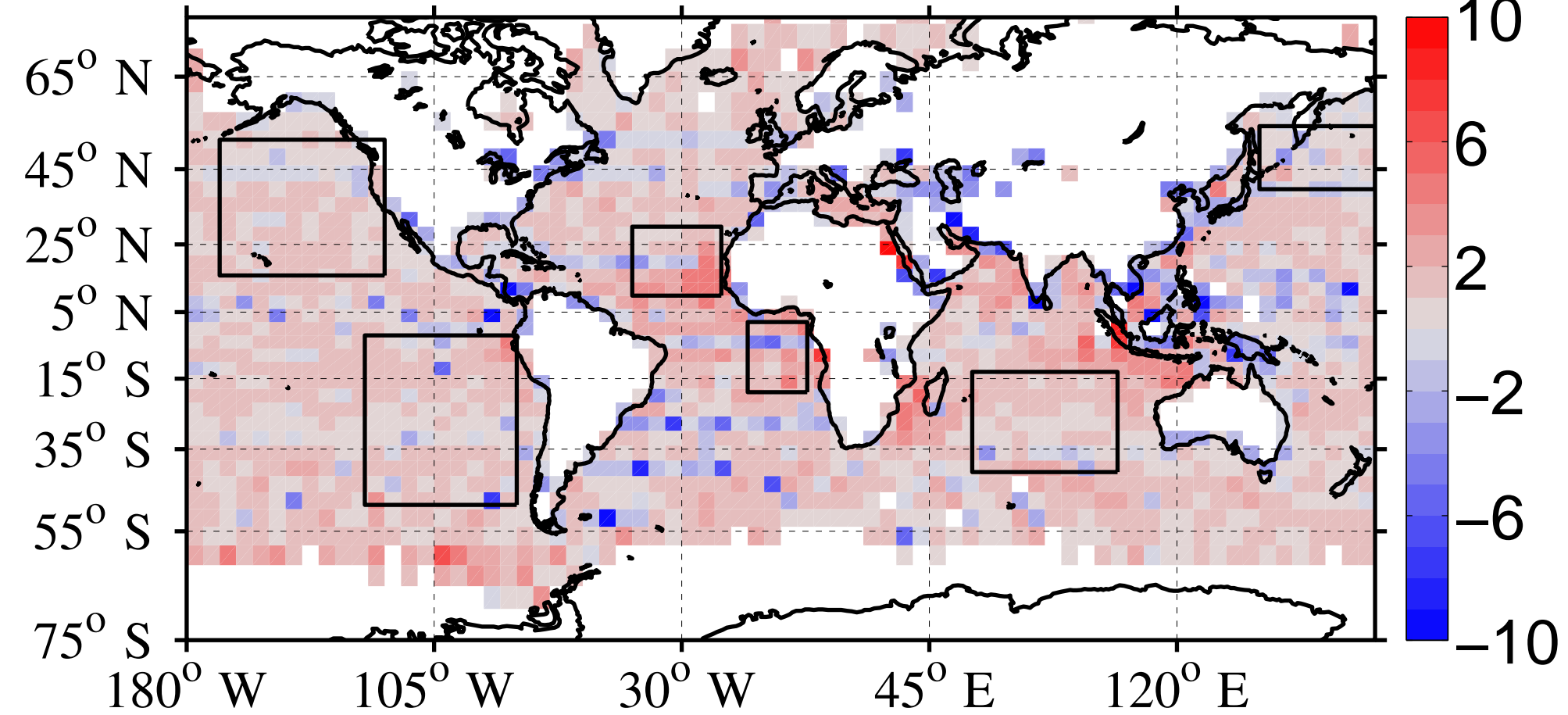
SON min: -21 max: 3 median: 1.02 mean: 0.62
