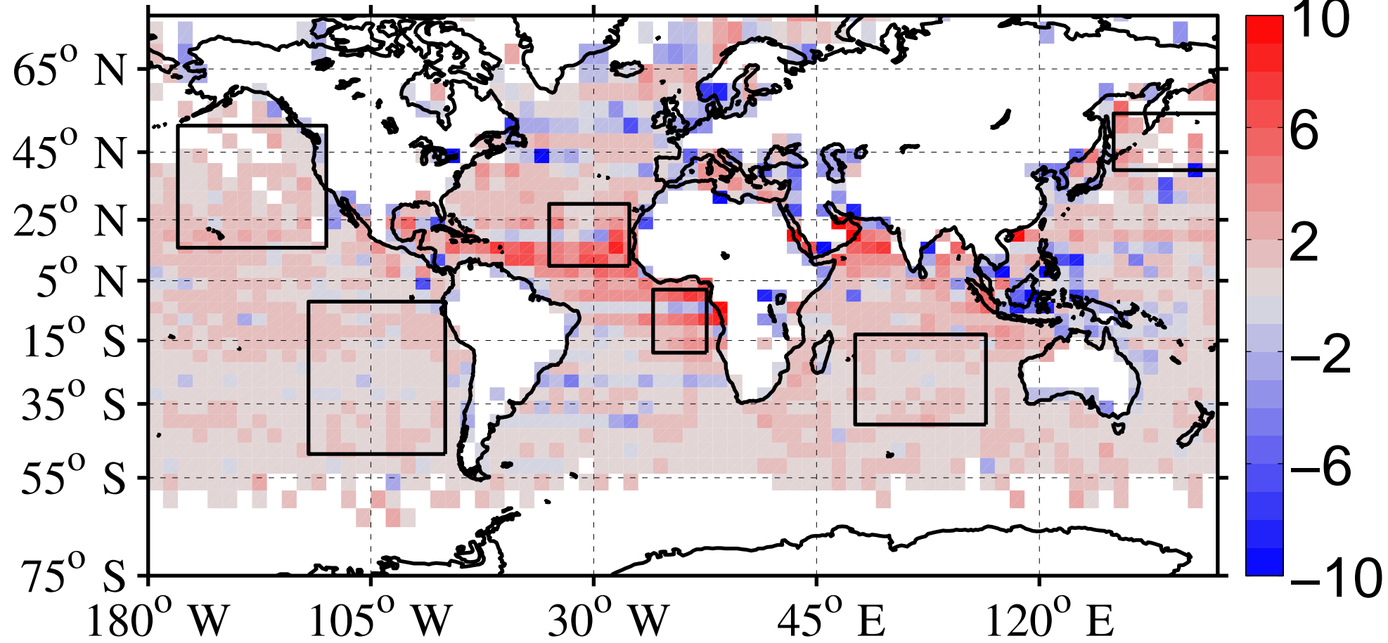
JJA min: -16 max: 5 median: 0.86 mean: 0.61
