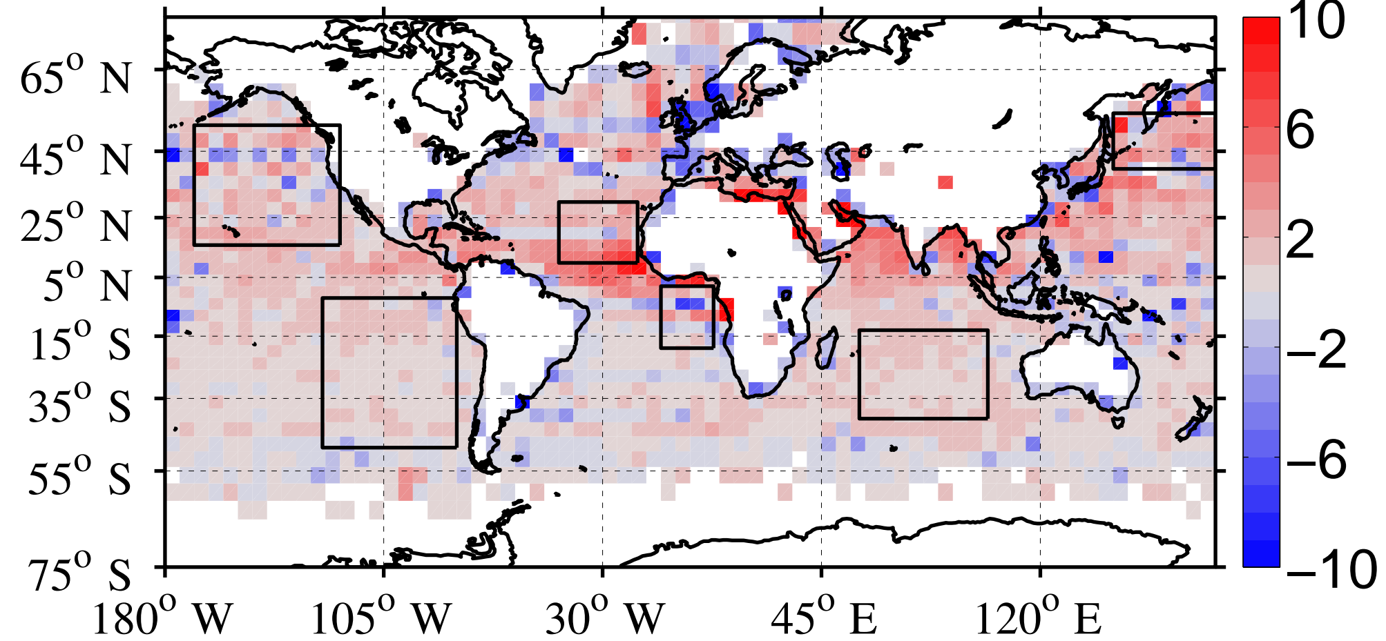
MAM min: -19 max: 5 median: 0.77 mean: 0.60
