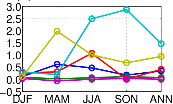
(c) CALIOP f_{AAC} (%)
