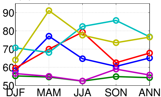
(c) CALIOP f_{AAC} (%)
