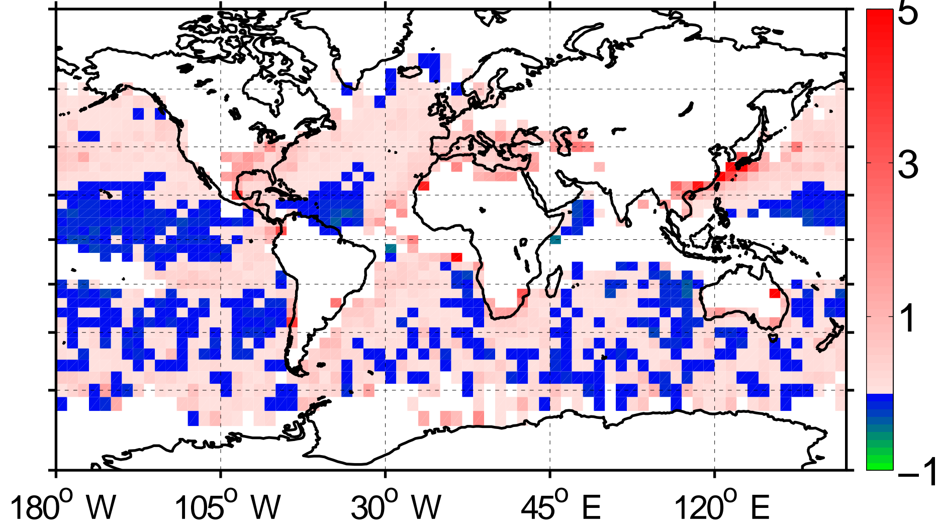
DJF min: -0.43 max: 5.87 mean: 0.13
