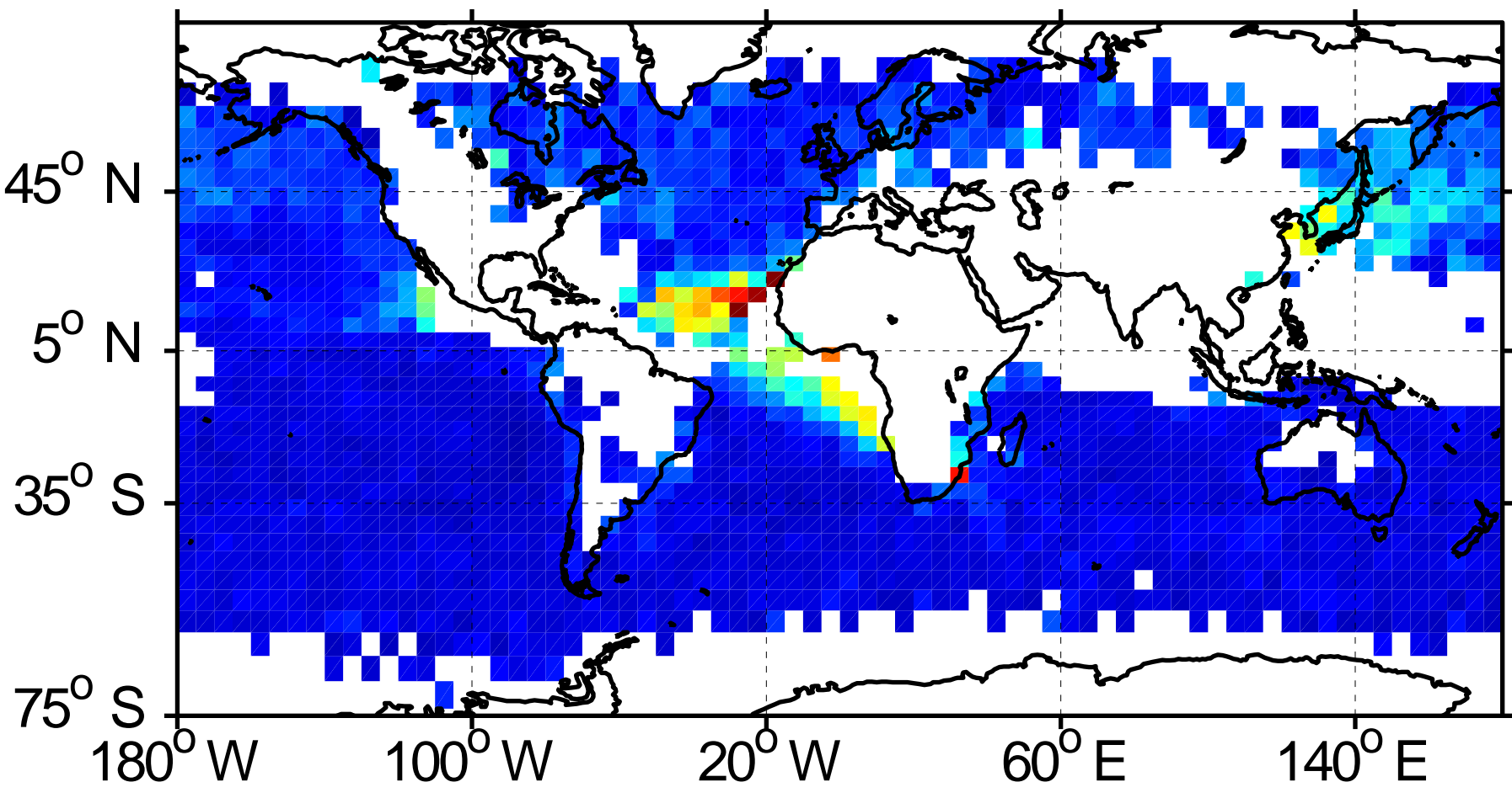
JJA max: 0.22 median: 0.02 mean: 0.04
