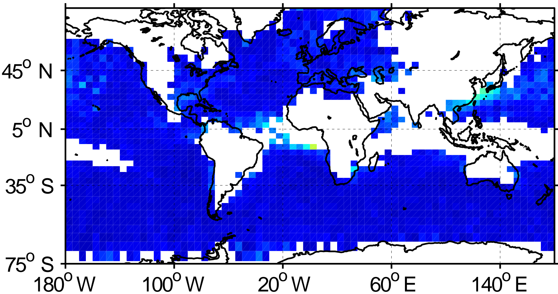
DJF max: 0.11 median: 0.02 mea: 0.03
