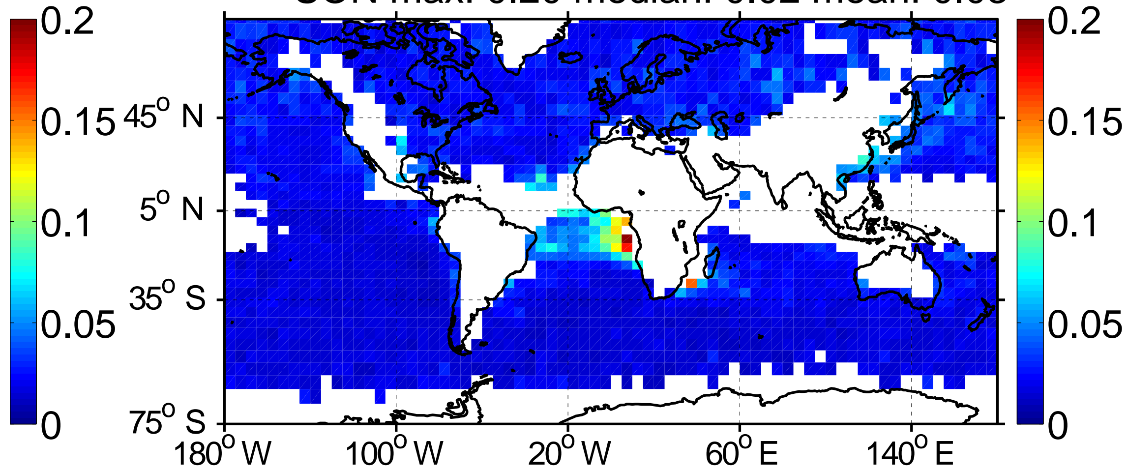
SON max: 0.20 median: 0.02 mean: 0.03
