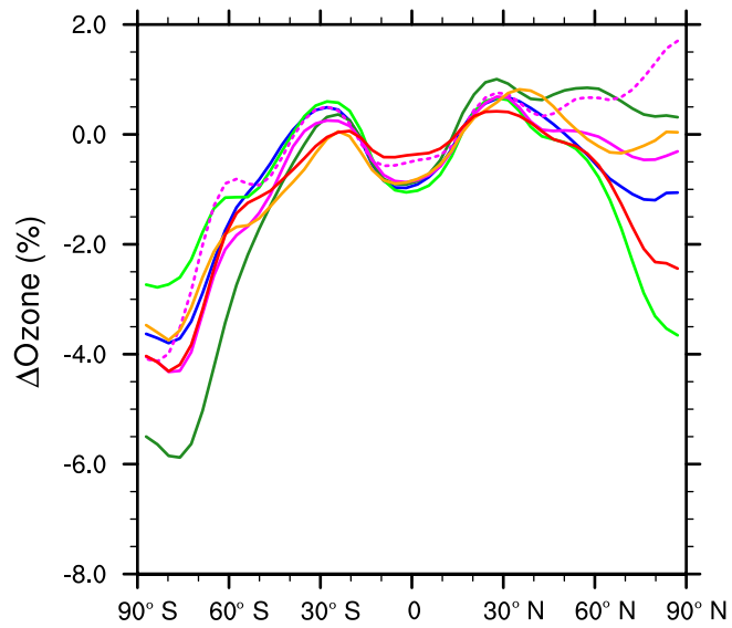
(f) Ozone depletion (SO 2 emission)
