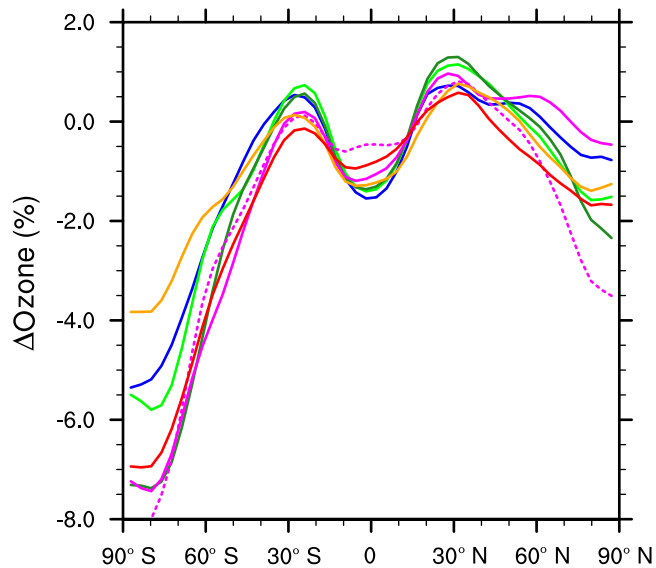
(e) Ozone depletion (AM H 2 SO 4 emission)
