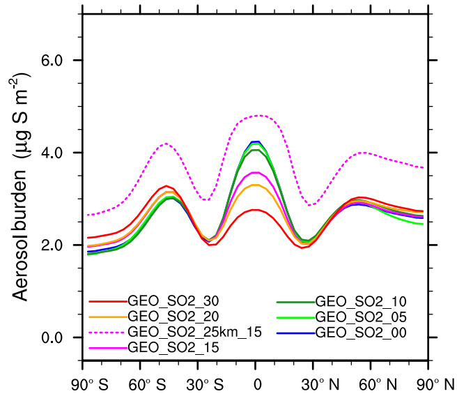
(b) Stratospheric aerosol burden (SO 2 emission)
