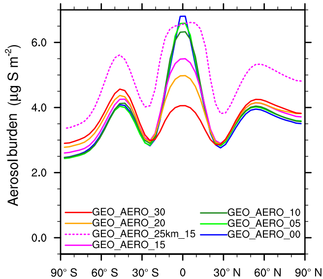
(a) Stratospheric aerosol burden (AM H 2 SO 4 emission)
