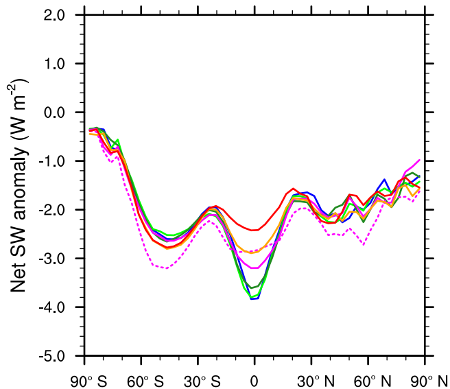
(c) Clear-sky SW forcing (AM H 2 SO 4 emission)
