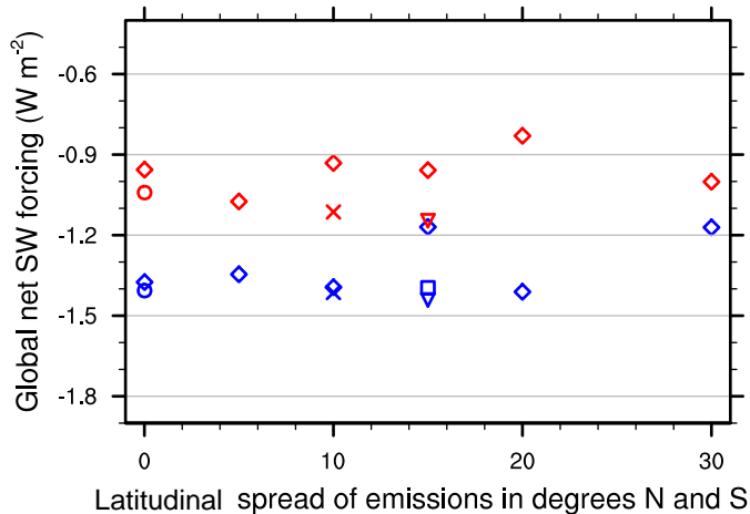
(c) All-sky SW radiative forcing
