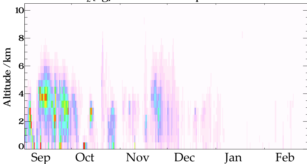
IASI SO 2 [Tg] - Holuhraun - 1 Sep 2014-28 Feb 2015
