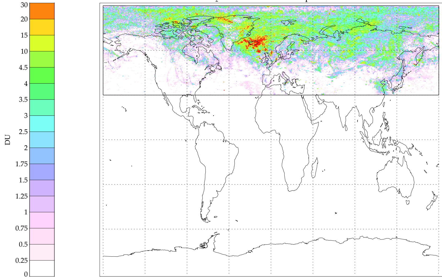
Maximum SO 2 column amount - 1 Sep 2014–28 Feb 2015
