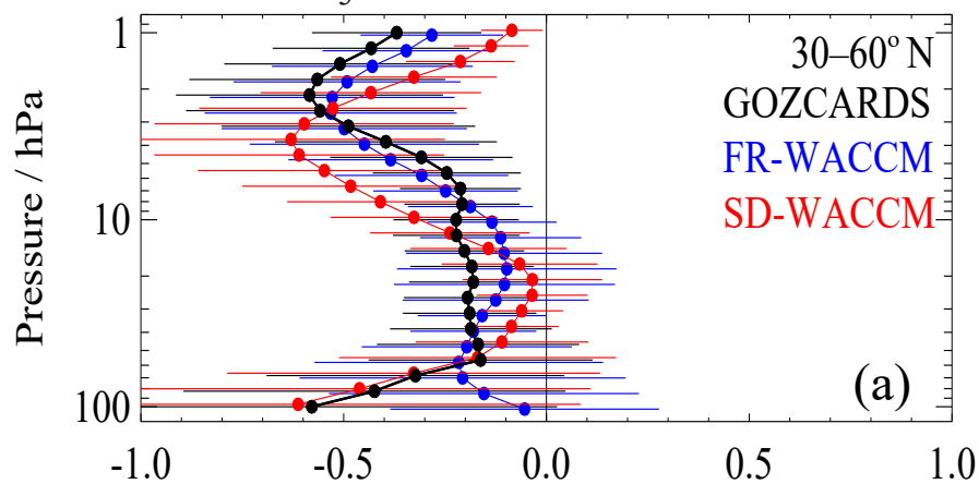
O 3 trends for 1985–1997
