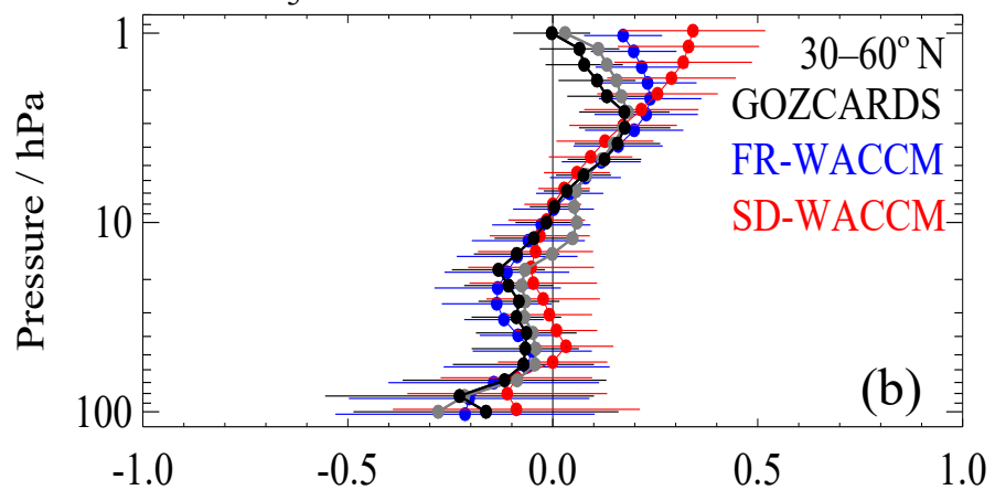
O 3 trends for 1998–2014/2018
