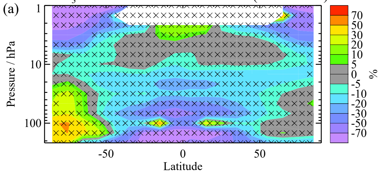
HNO 3 % Dif.: SD-WACCM - MLS (2005–2014)
