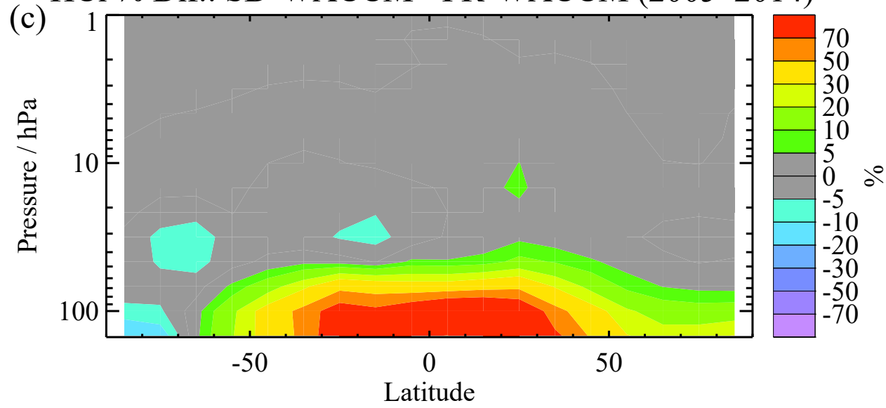
HCl % Dif.: SD-WACCM - FR-WACCM (2005–2014)
