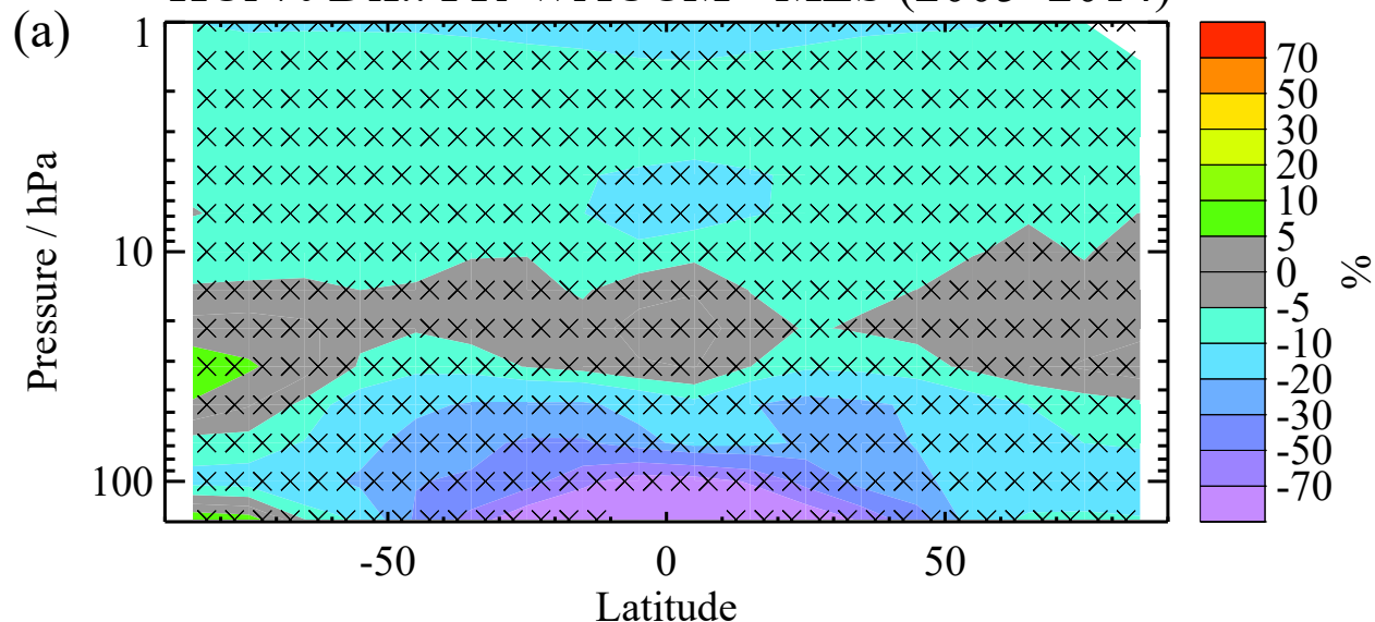
HCl % Dif.: SD-WACCM - MLS (2005–2014)
