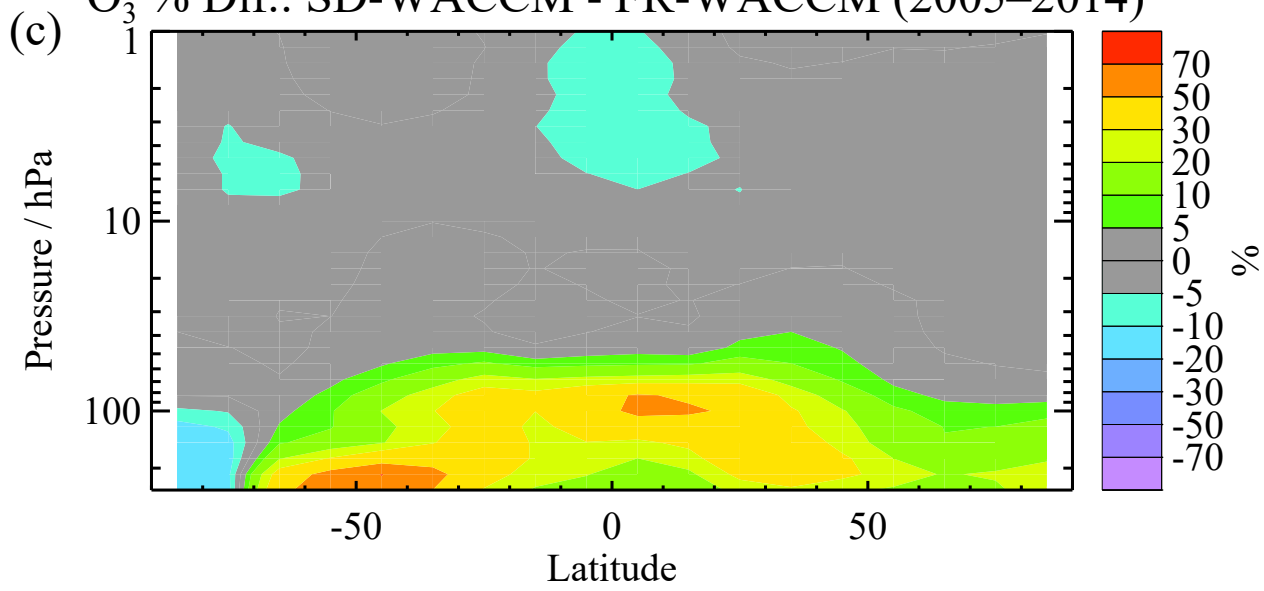
O 3 % Dif.: SD-WACCM - FR-WACCM (2005–2014)
