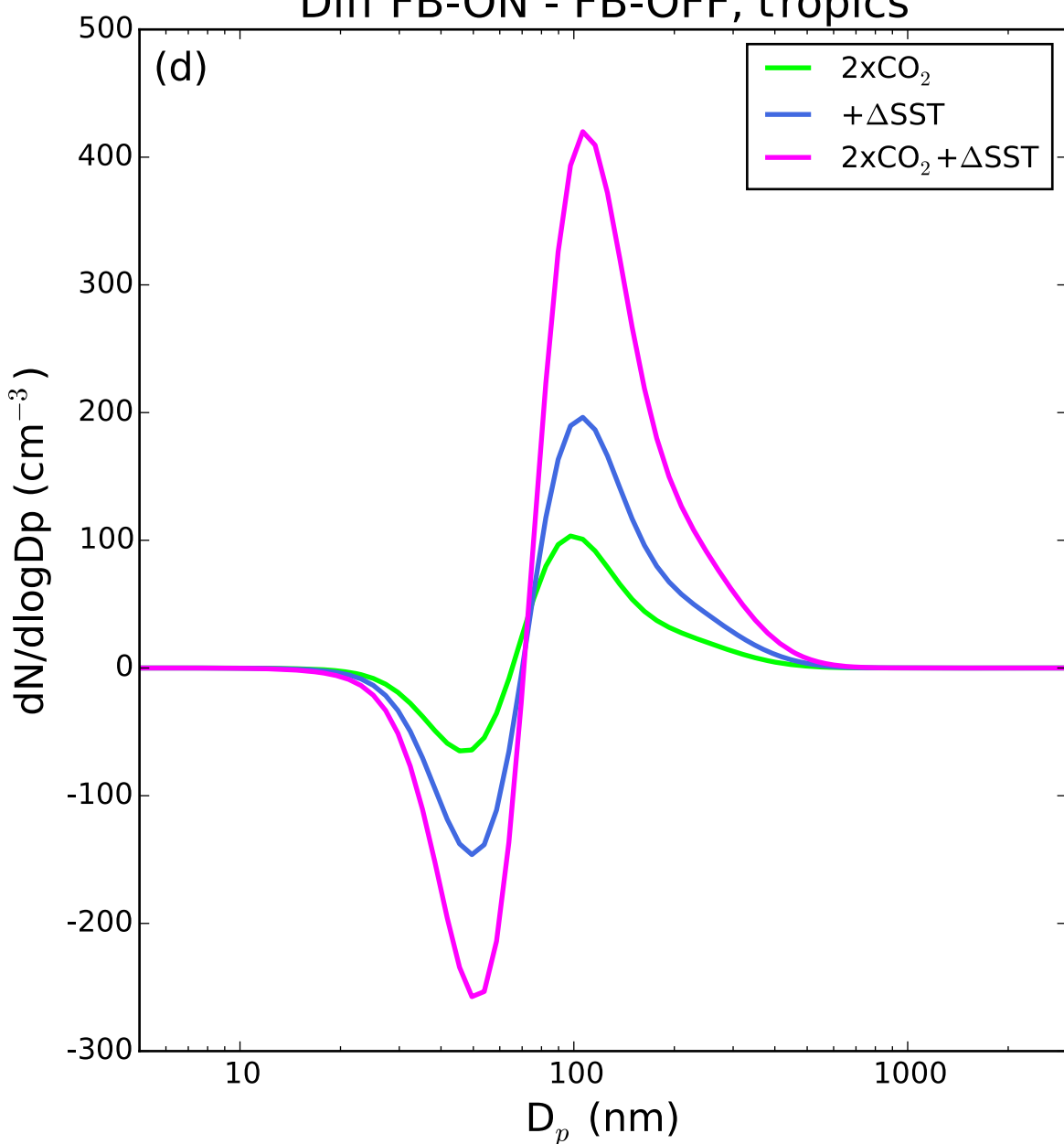
Diff FB-ON - FB-OFF, tropics
