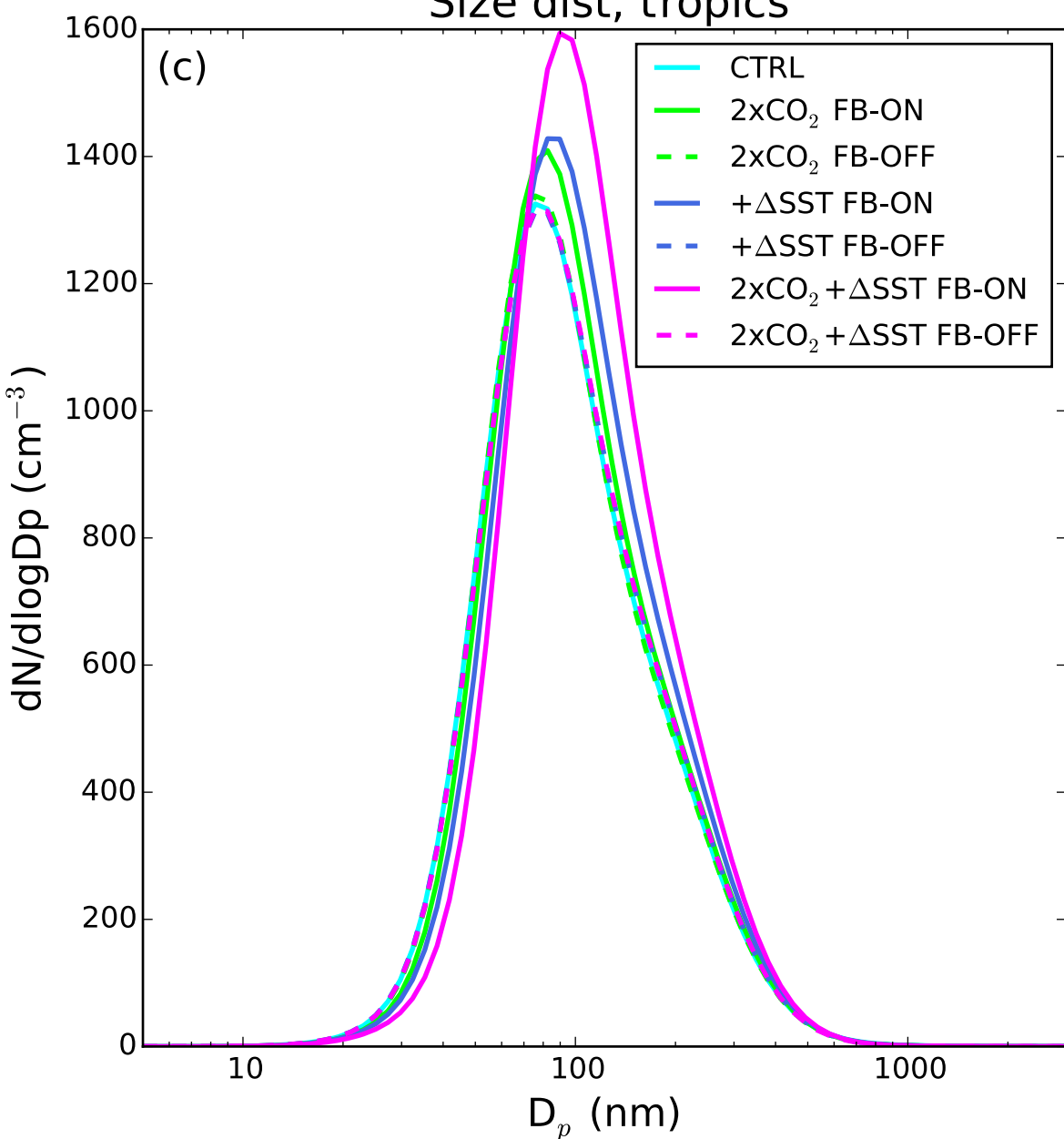
Size dist, tropics
