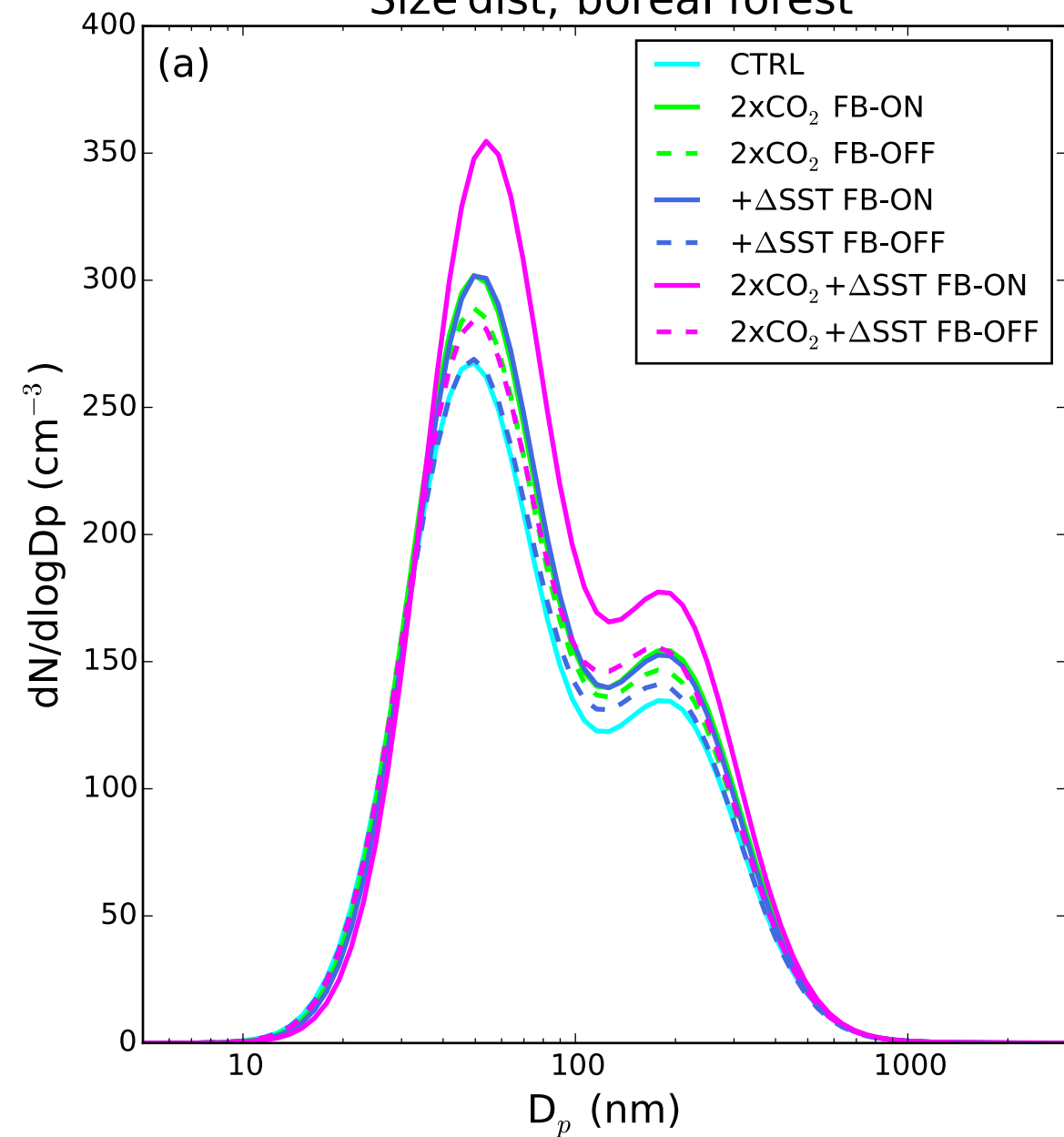
Size dist, boreal forest
