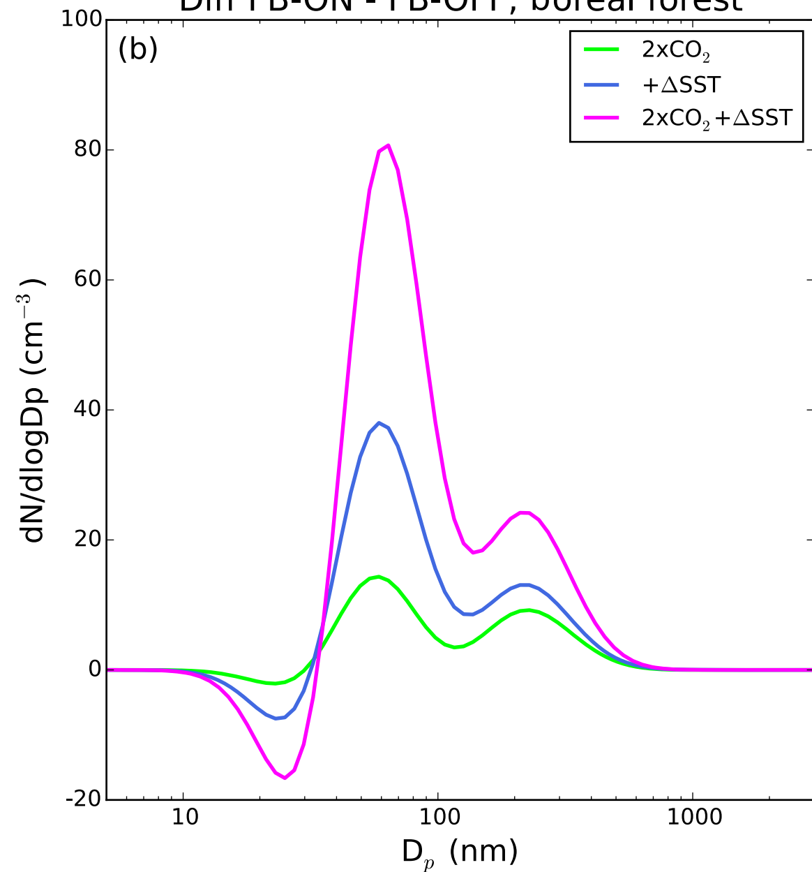
Diff FB-ON - FB-OFF, boreal forest
