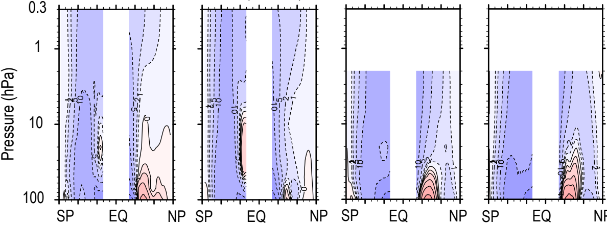
\Psi_{GW} (MERRA-2)
