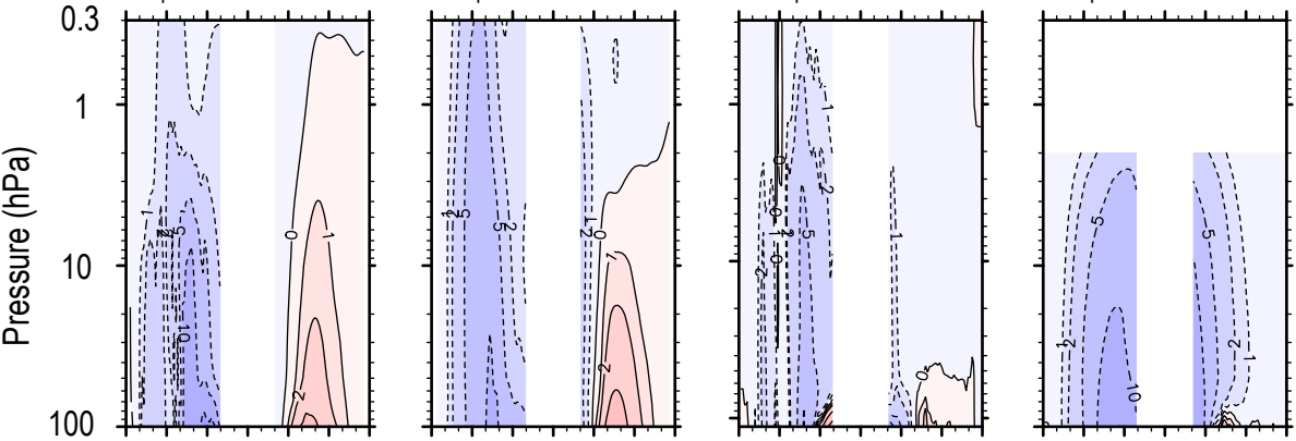
\Psi_{pGW} (MERRA-2)
