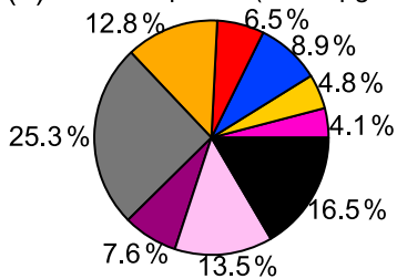
(b) Pollution period ( 38.37 \mu\text{g m}^{-3} )
