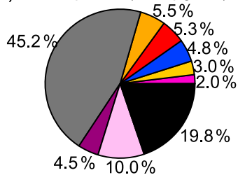
(a) Clean period ( 2.62 \mu\text{g m}^{-3} )
