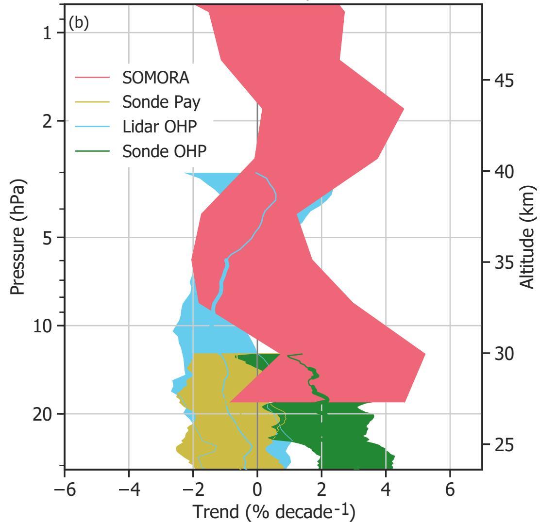
Trends 1997–2017, Payerne and OHP
