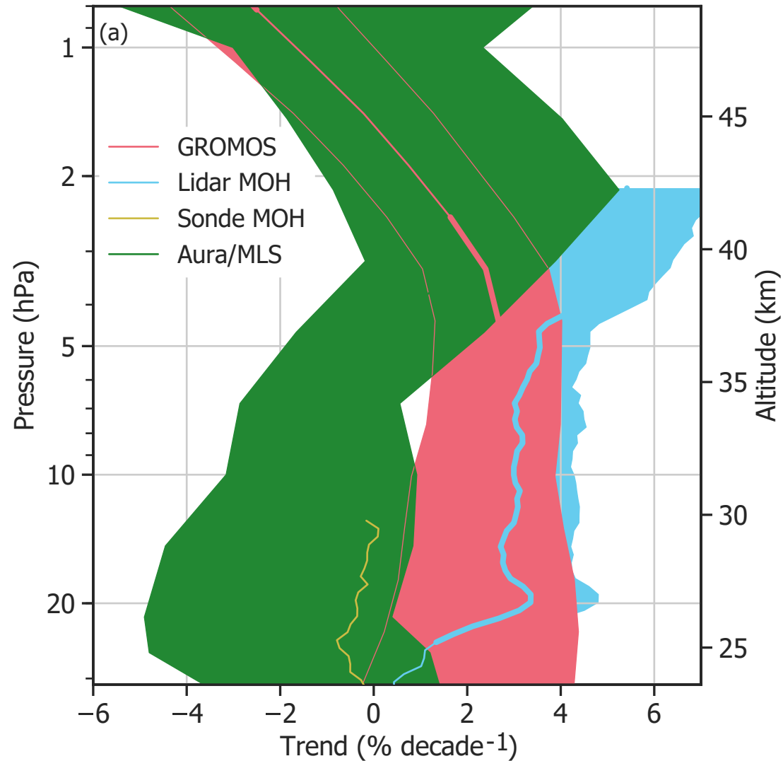
Trends 1997–2017, Bern, MOH, and Aura/MLS
