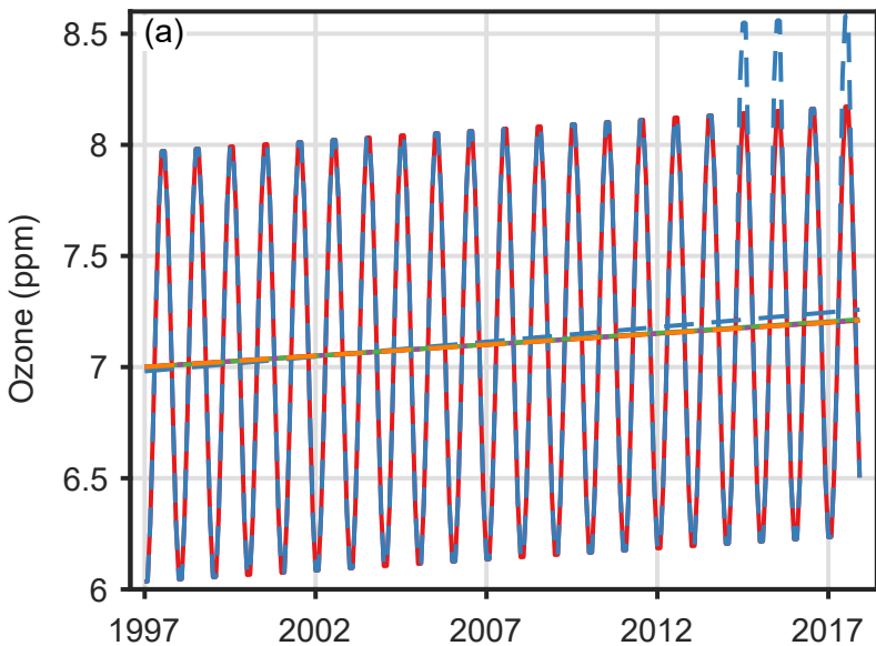
Trends for different artificial time series
