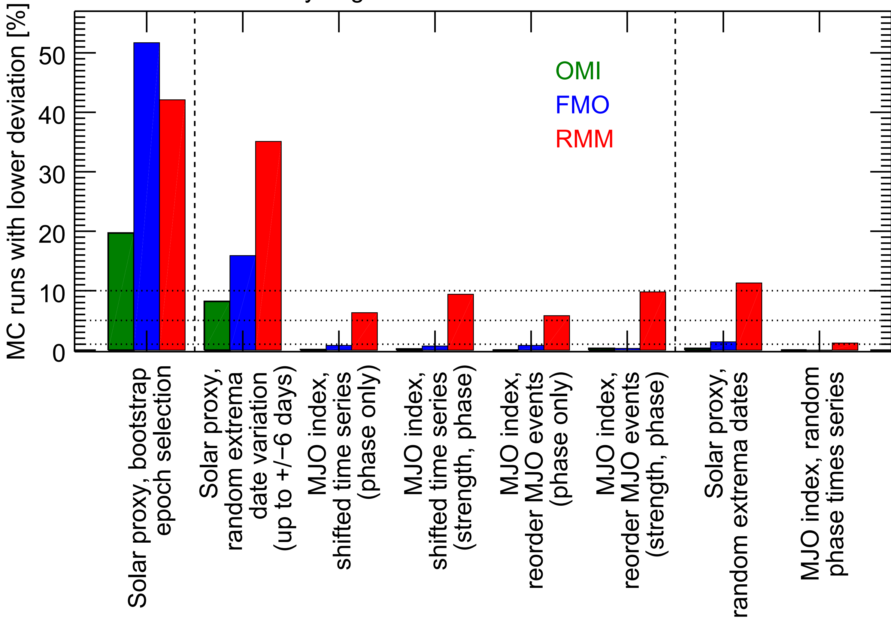
Probability to get lower deviations with random data
