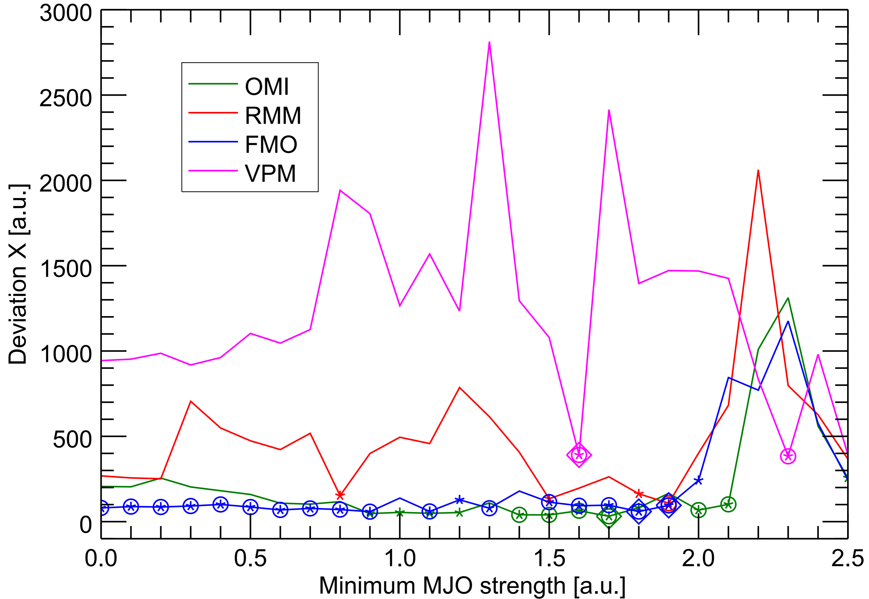
Setup: QBO east, winter, solar minimum, Lyman alpha
