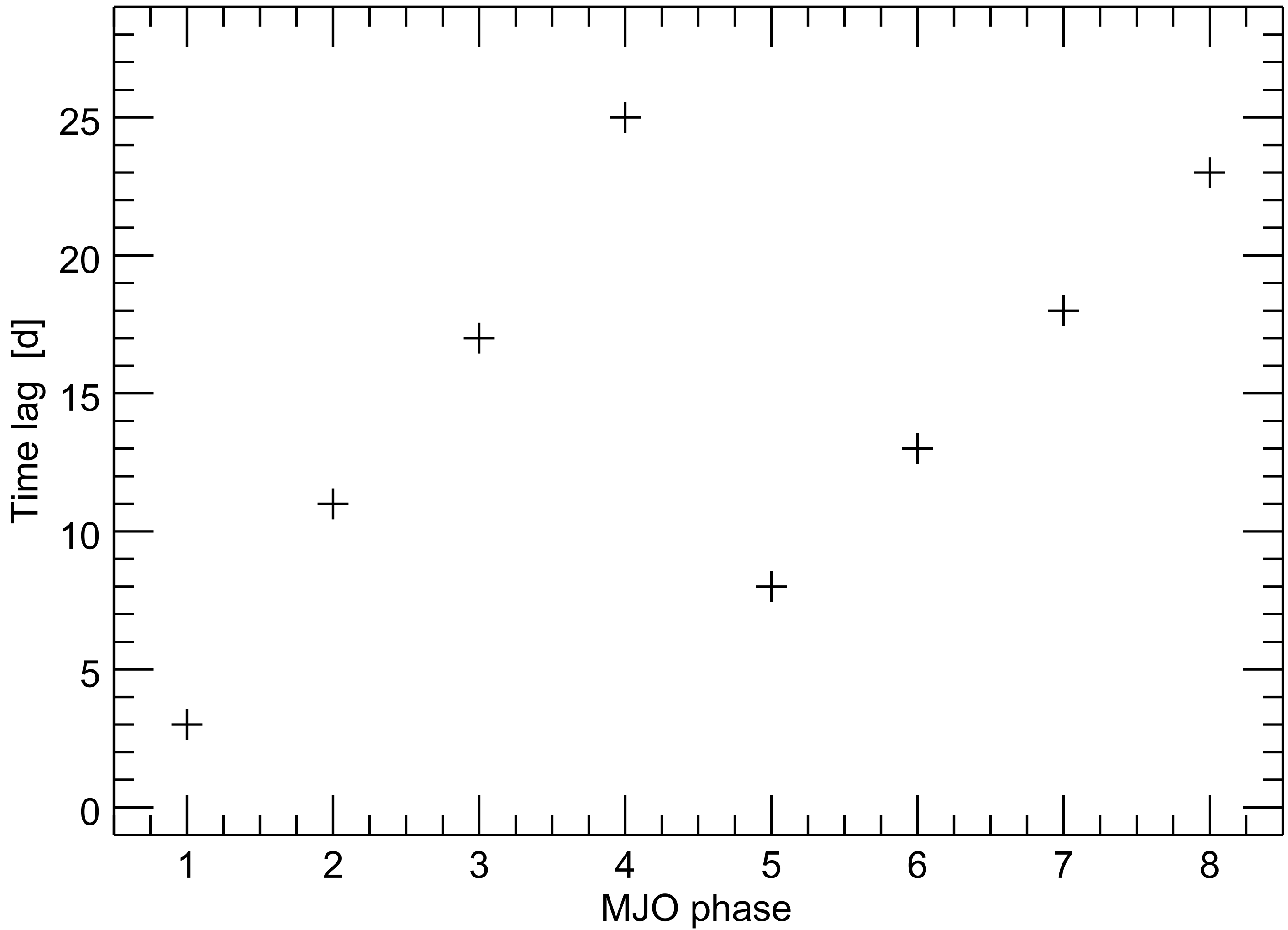
Time lags with max. MJO phase occurrence
