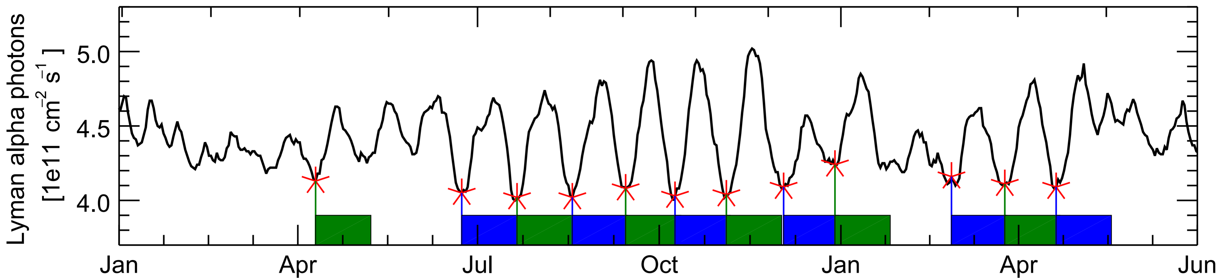
(a) Lyman alpha solar proxy
