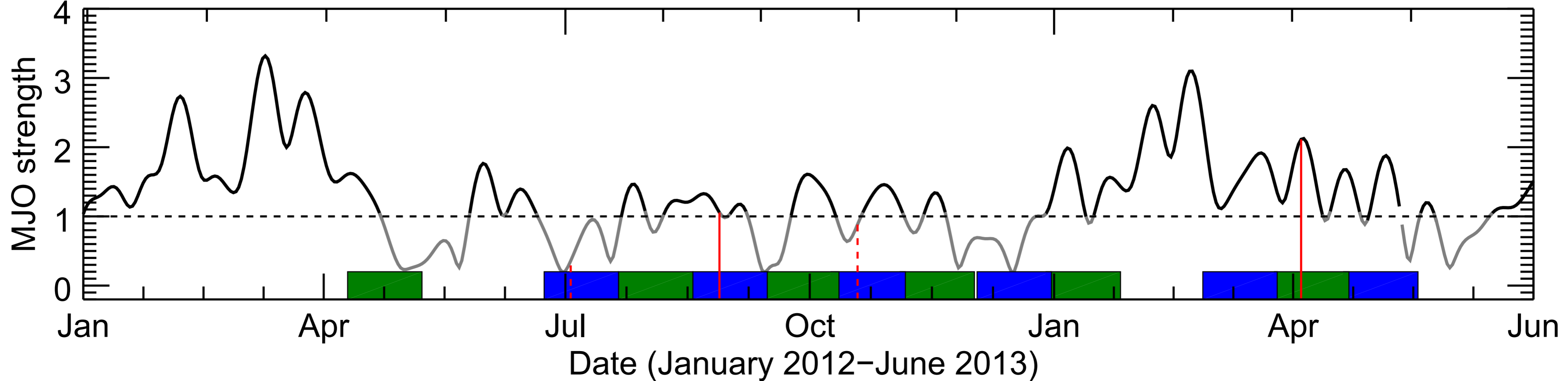
(c) MJO strength
