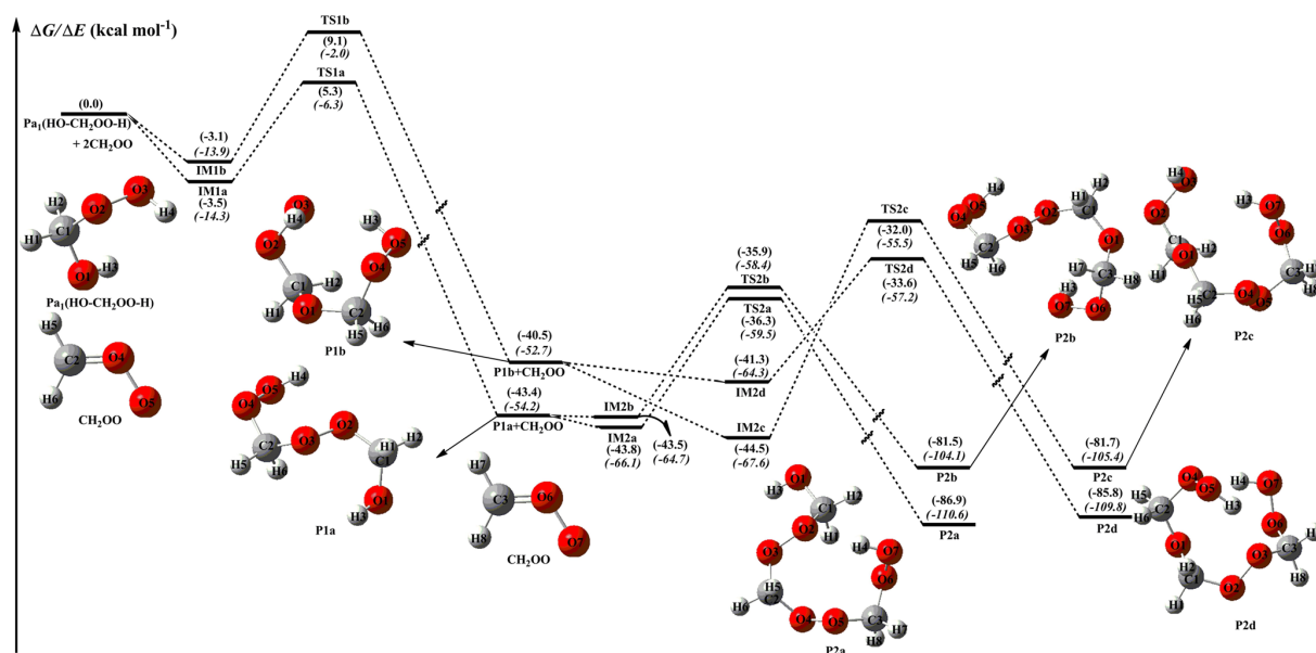
Figure 2. PES ( \Delta G and \Delta E , in italics) for the reaction of \text{CH}_2\text{OO} with \text{HO-CH}_2\text{OO-H} ( \text{Pa}_1 ) computed at the M06-2X/def2-TZVP//M06-2X/6-311+G(2df,2p) level of theory.
