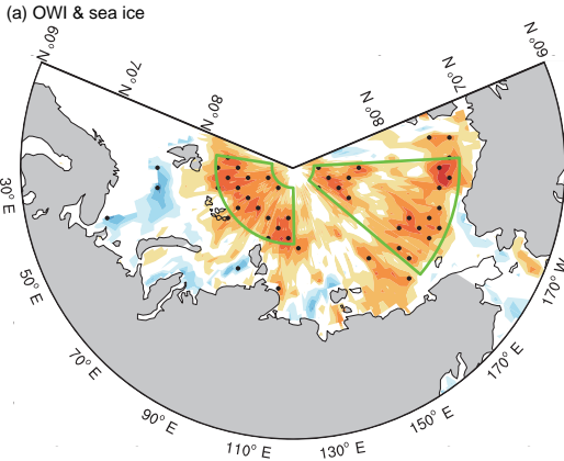
(a) OWI & sea ice
