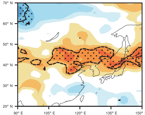
(e) UVB & mcc and lcc
