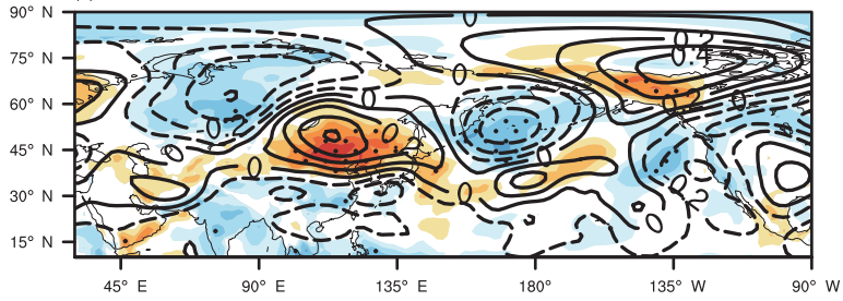
(c) SAT & Z500
