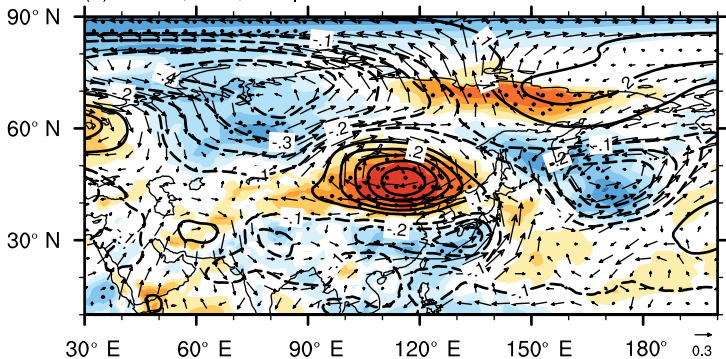
(a) UV200,Z500,SAT | OWI
