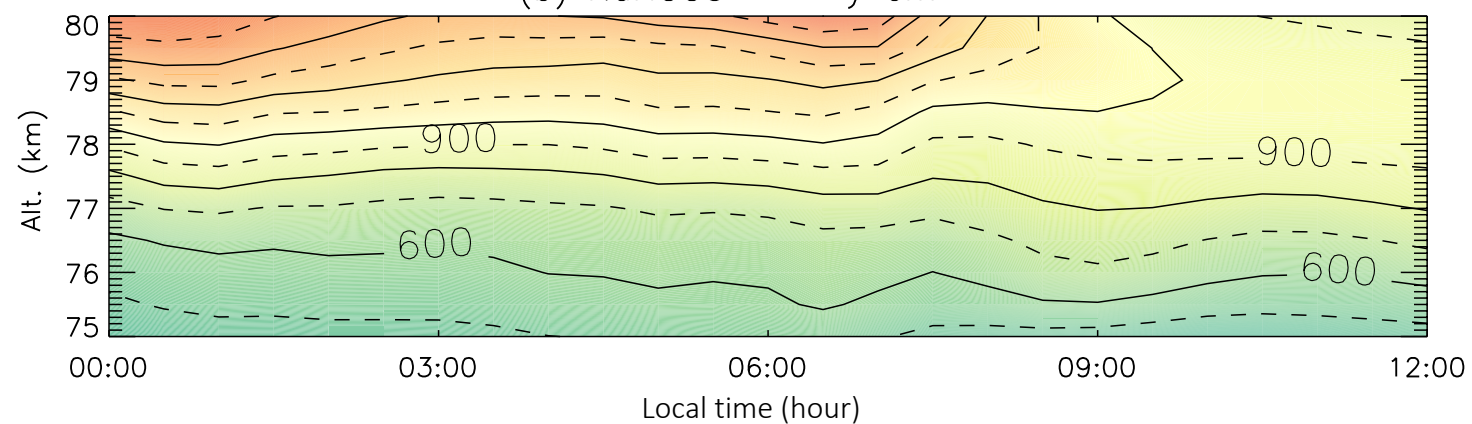
(c) H density \text{cm}^{-3}
