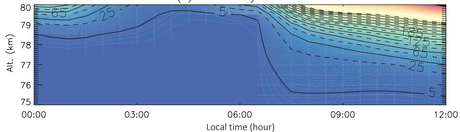
(b) \text{NaHCO}_3 density \text{cm}^{-3}
