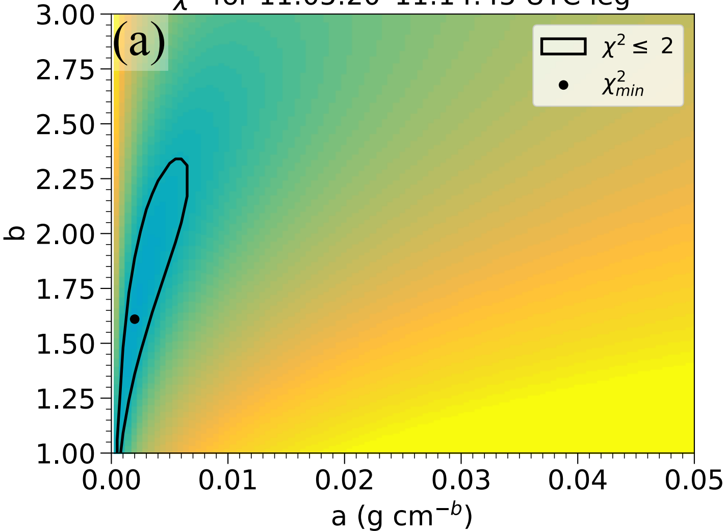
\chi^2 for 11:05:20–11:14:45 UTC leg
