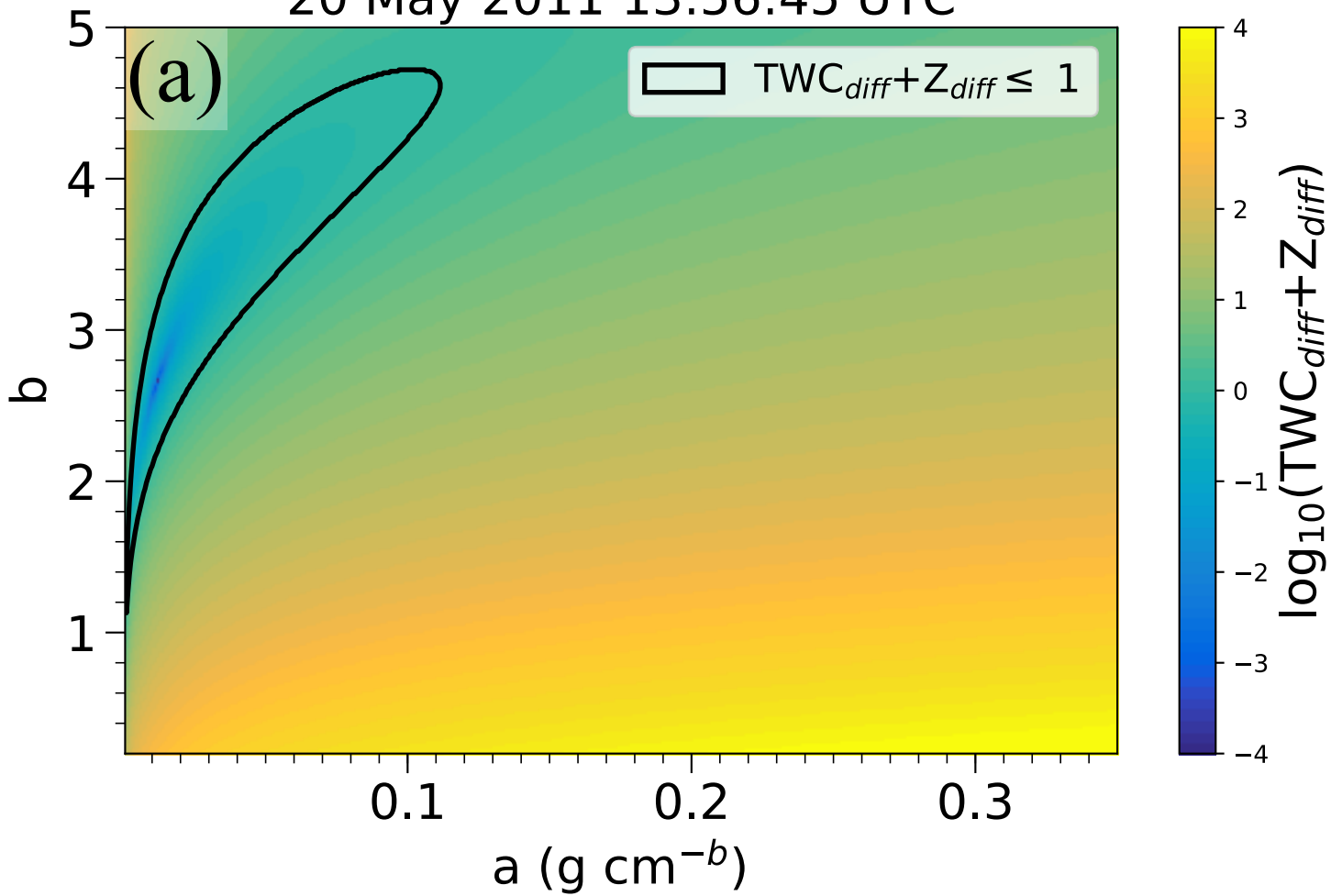
TWC diff +Z diff for coincident point 20 May 2011 13:56:45 UTC
