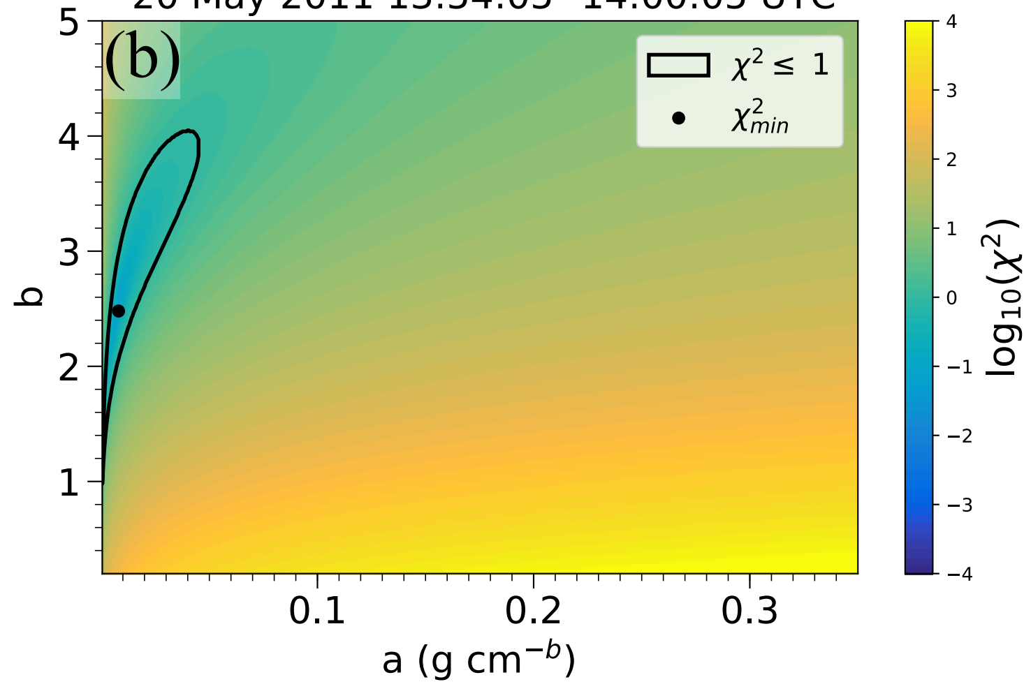
\chi^2 for flight leg 20 May 2011 13:54:05–14:00:05 UTC
