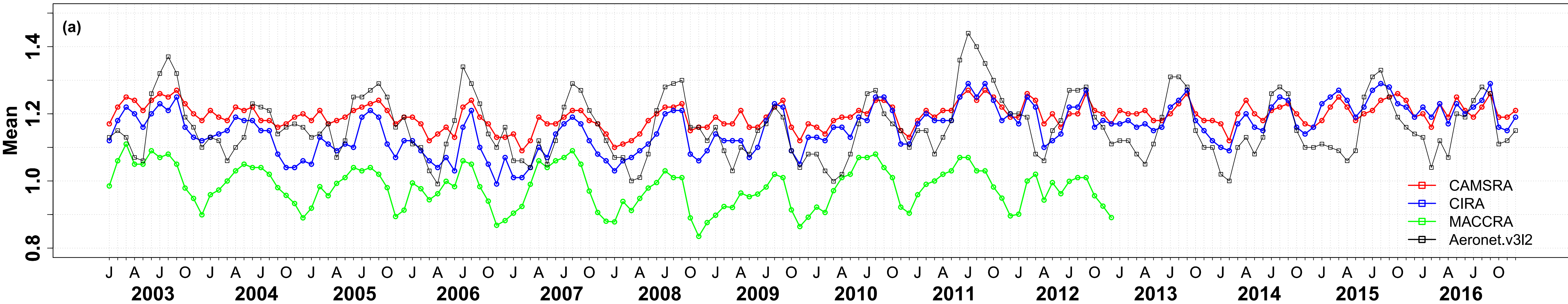
MACC/CAMS 2003–2016 versus Aeronet – Ångström exponent
