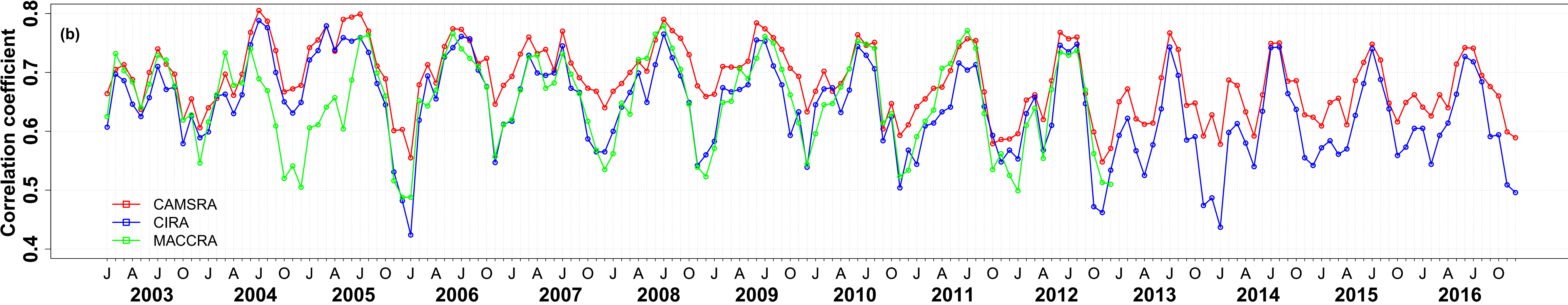
MACC/CAMS reanalysis 2003–2016 versus Aeronet – Ångström exponent
