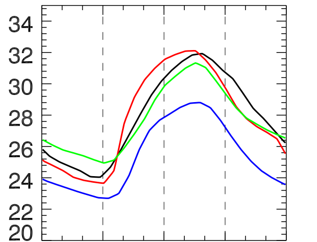
Temperature / °C
