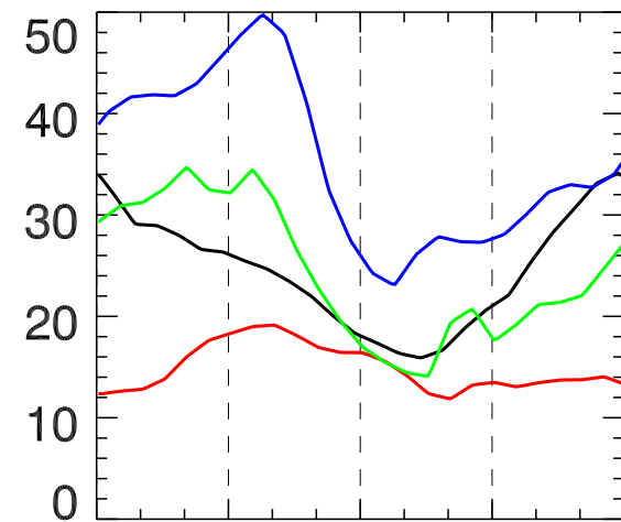
AHC / ppbv
